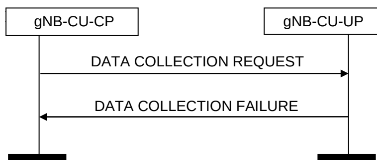
Figure 8.2.11.3-1: Data Collection Reporting Initiation, unsuccessful operation
