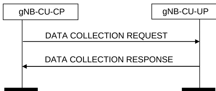
Figure 8.2.11.2-1: Data Collection Reporting Initiation, successful operation
