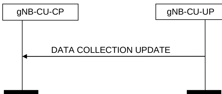
Figure 8.2.12.2-1: Data Collection Reporting, successful operation
