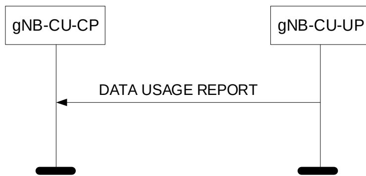
Figure 8.3.8.2-1: Data Usage Report procedure: Successful Operation.
