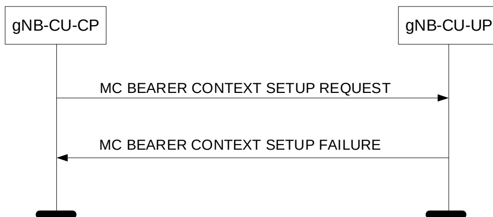
Figure 8.6.2.1.3-1: MC Bearer Context Setup procedure: Unsuccessful Operation.
