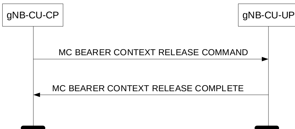
Figure 8.6.2.4.2-1: MC Bearer Context Release procedure: Successful Operation.
