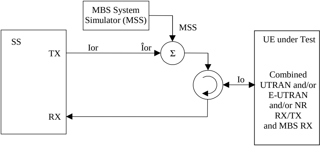
Figure A.6: Connection for MBS Minimum Performance requirements tests for UE with combined UTRAN and/or E-UTRAN and/or NR and MBS antenna
