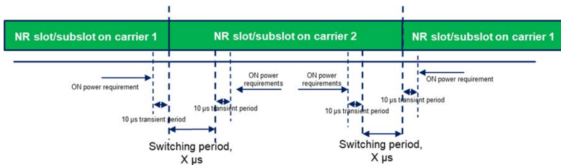
Figure 6.3C.3.1-1b: Time mask for switching between SUL carrier 1 and UL Carrier 2, where the switching period is located in carrier 2
