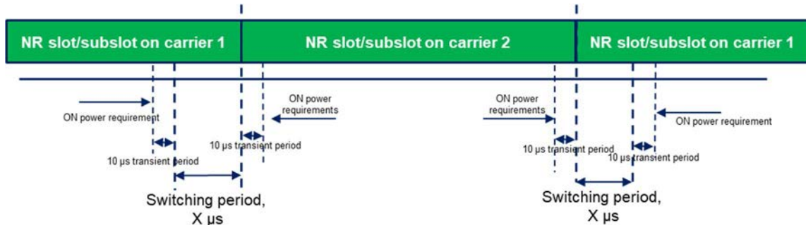
Figure 6.3C.3.2-1a: Time mask for switching between SUL carrier 1 and UL Carrier 2, where the switching period is located in carrier 1
