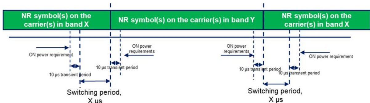
Figure 6.3A.3.3.6-1: Time mask for switching between band X and band Y, where the switching period is located in band X
