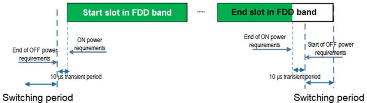
Figure 6.3A.3.3.7-1: ON/OFF time mask for NR UL transmission for DL CA via switching with non-CA in the UL
