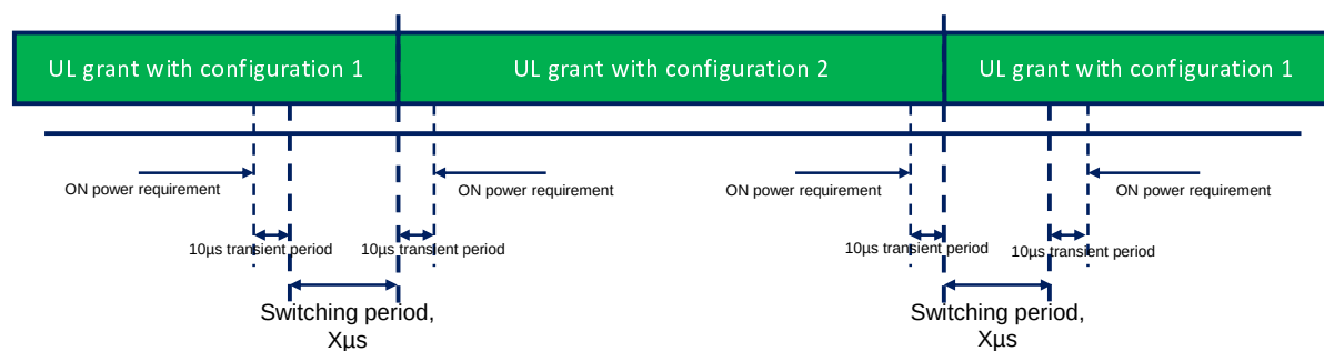
Figure 6.3A.3.3.8-1a: Time mask for switching between UL Configuration 1 and UL Configuration 2, where the switching period is located in Configuration 1
