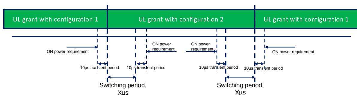
Figure 6.3A.3.3.8-1b: Time mask for switching between UL Configuration 1 and UL Configuration 2, where the switching period is located in Configuration 2
