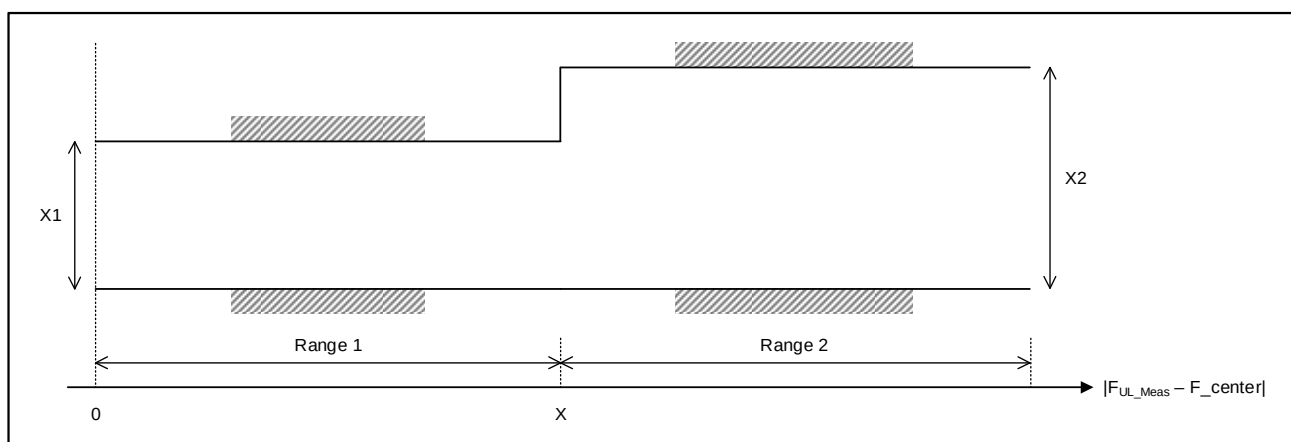
Figure 6.4.2.4.2-1: The limits for EVM equalizer spectral flatness referenced in table 6.4.2.4.2-1.
