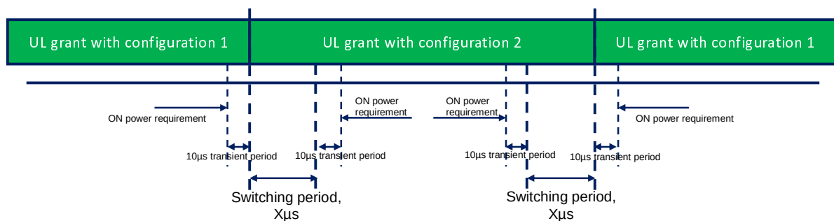
Figure 6.3A.3.3.8-1b: Time mask for switching between UL Configuration 1 and UL Configuration 2, where the switching period is located in Configuration 2
