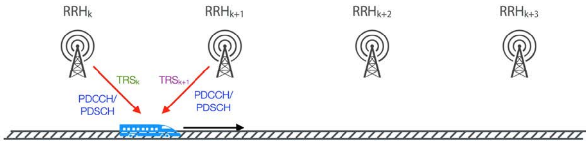
Figure B.3.6-1: Deployment of HST-SFN Scheme B
