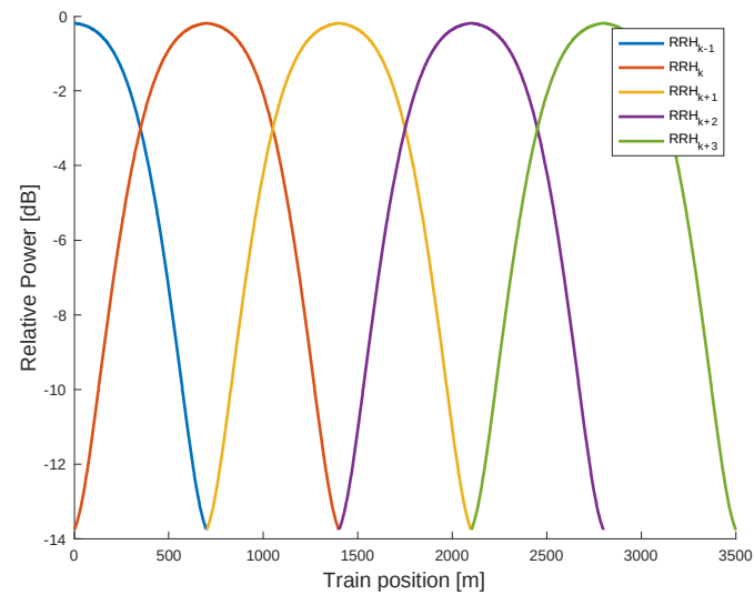
Figure B.3.5-2 Relative power level trajectories
