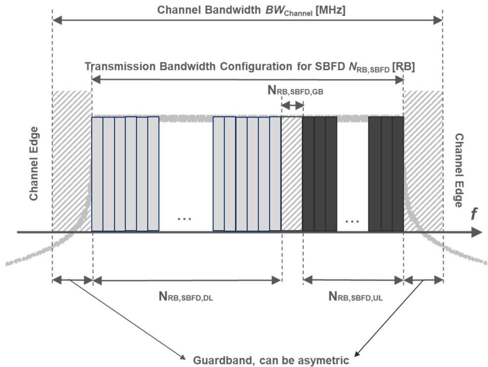
Figure 5.3.1-3: Definition of channel bandwidth and transmission bandwidth configuration for SBFD DU operation
