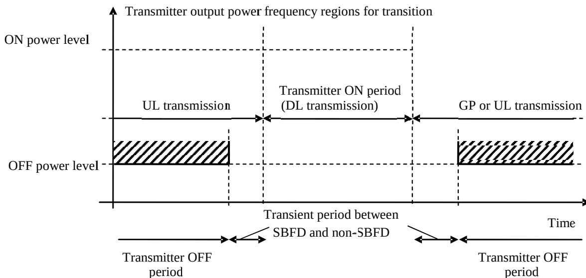
Figure 12.5.10.1-1: Example of relations between transmitter ON period, transmitter OFF period and transmitter transient period between SBFD and non-SBFD operation
