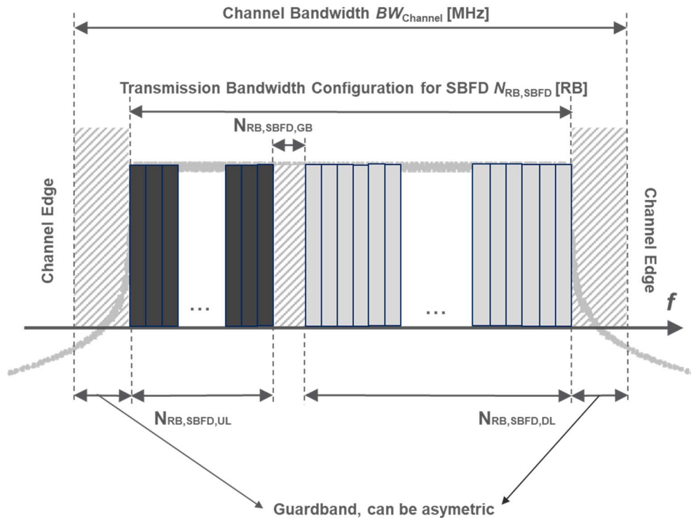
Figure 5.3.1-4: Definition of channel bandwidth and transmission bandwidth configuration for SBFD UD operation
