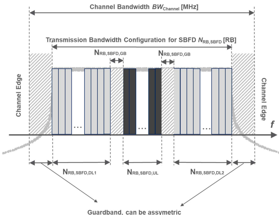
Figure 5.3.1-2: Definition of channel bandwidth and transmission bandwidth configuration for SBFD DUD operation
