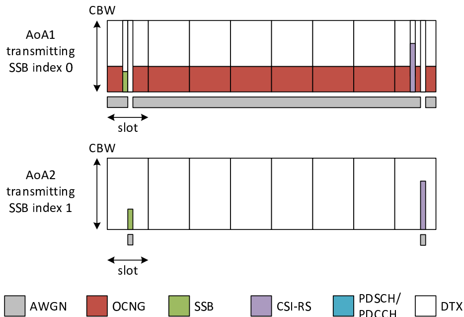
Figure A.5.5.1.2.1-2: Time multiplexed downlink transmissions
