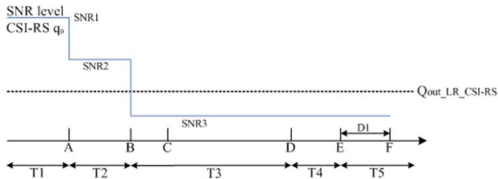
Figure A.6.5.4.1-1: SNR variation for CSI-RS-based beam failure detection and link recovery testing in DRX mode
