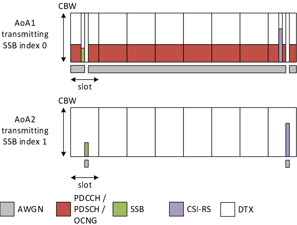
Figure A.5.5.8.1.1.1-1: Time multiplexed downlink transmissions during T1
