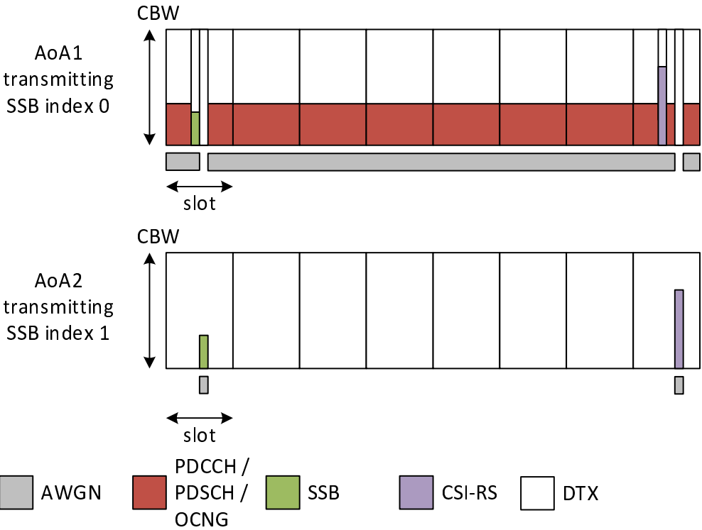
Figure A.5.5.8.1.1.1-1: Time multiplexed downlink transmissions during T1
