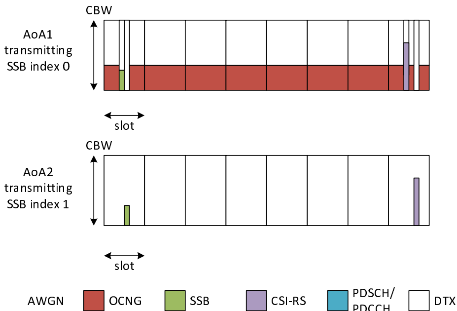
Figure A.5.6.1.1-1: Time multiplexed downlink transmissions (Config 1,2 example)
