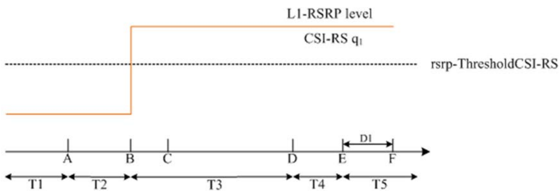
Figure A.6.5.5.4.1-2: L1-RSRP level variation for CSI-RS based beam failure detection and link recovery testing in DRX mode
