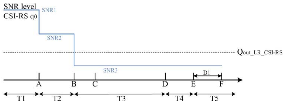
Figure A.7.5.5.4.1-1: SNR variation for CSI-RS-based beam failure detection and link recovery testing in DRX mode
