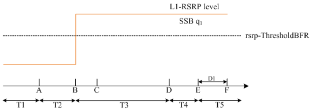
Figure A.6.5.5.6.1-2: L1-RSRP level variation for beam failure detection and link recovery testing for SCell in DRX mode
