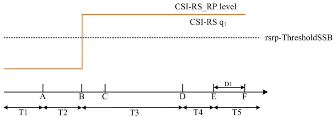
Figure A.5.5.7.1-2: CSI-RS_RP level variation for CSI-RS based beam failure detection and link recovery testing for SCell in DRX mode
