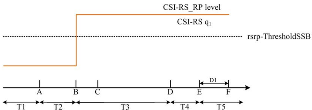
Figure A.7.5.5.7.1-2: CSI-RS_RP level variation for CSI-RS based beam failure detection and link recovery testing for SCell in DRX mode
