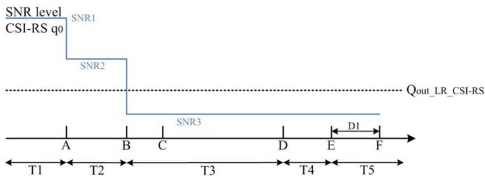
Figure A.5.5.6.1-1: SNR variation for CSI-RS based beam failure detection and link recovery testing for SCell in non-DRX mode
