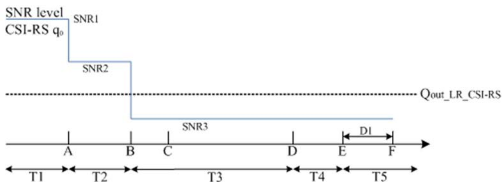
Figure A.4.5.5.1-1: SNR variation for beam failure detection and link recovery testing for SCell in non-DRX mode
