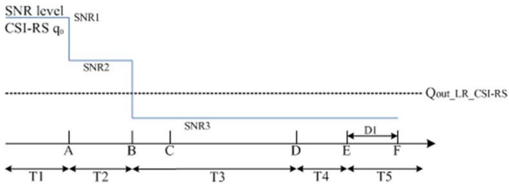
Figure A.6.5.5.6.1-1: SNR variation for beam failure detection and link recovery testing for SCell in DRX mode
