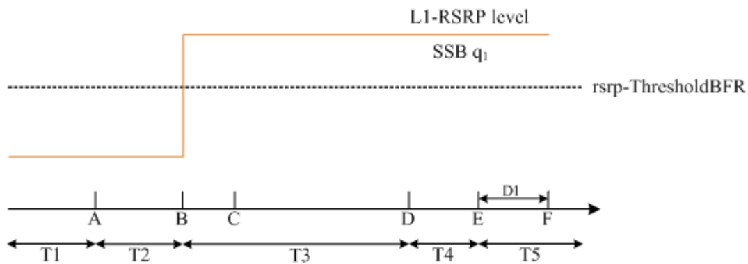
Figure A.6.5.5.1-2: L1-RSRP level variation for beam failure detection and link recovery testing for SCell in non-DRX mode
