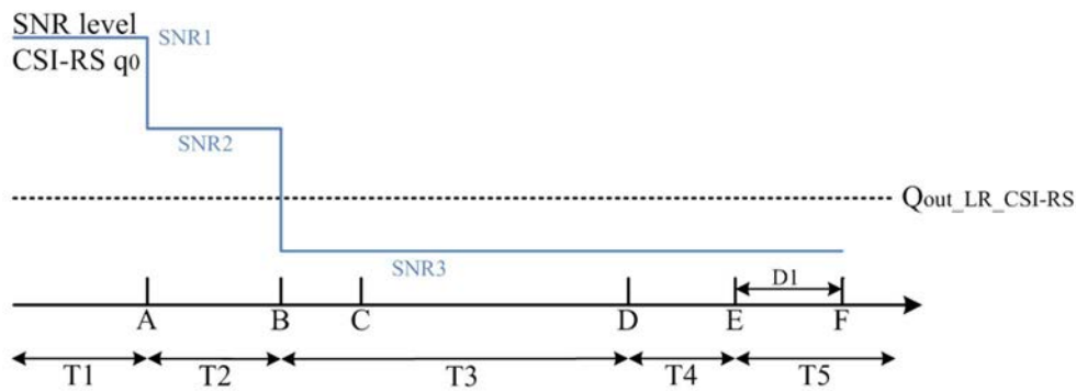
Figure A.7.5.5.7.1-1: SNR variation for beam failure detection and link recovery testing for SCell in DRX mode
