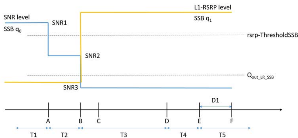
Figure A.10.3.4.2.1-1: SNR and L1-RSRP variation for SSB-based beam failure detection and link recovery testing in DRX mode
