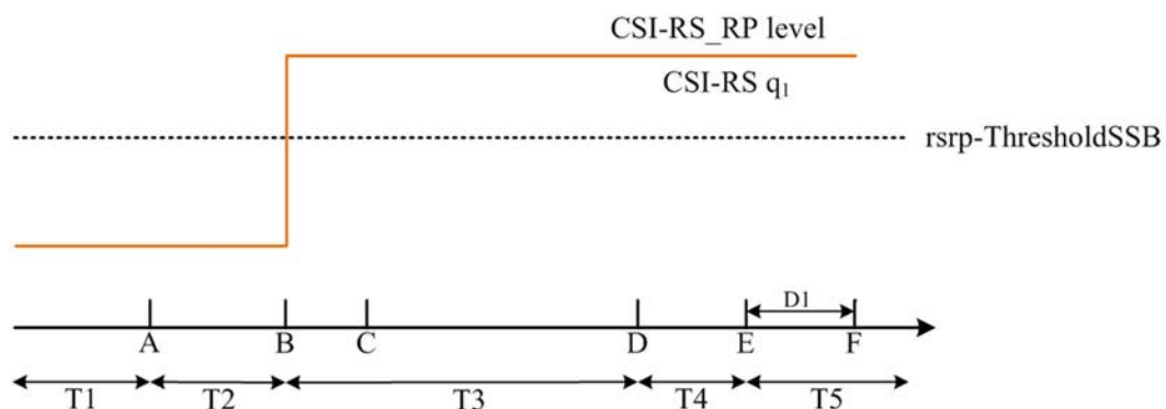
Figure A.7.5.5.6.1-2: CSI-RS_RP level variation for CSI-RS based beam failure detection and link recovery testing for SCell in non-DRX mode
