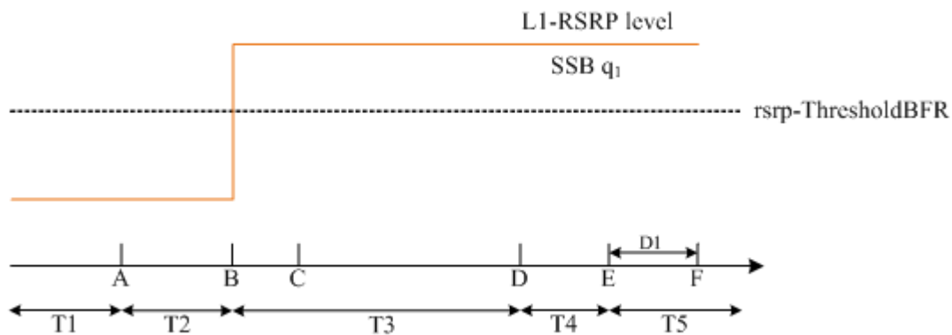
Figure A.4.5.5.1-2: L1-RSRP level variation for beam failure detection and link recovery testing for SCell in non-DRX mode
