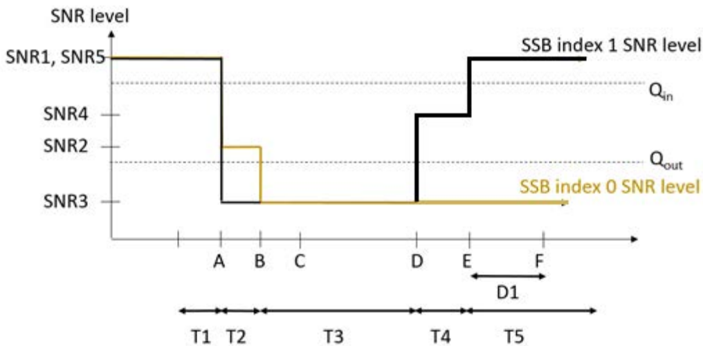
Figure A.7.5.1.2.1-1: SNR variation for in-sync testing
