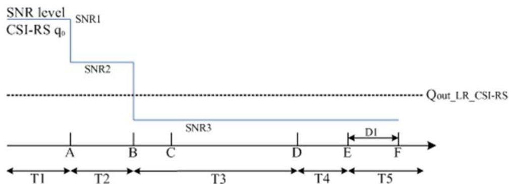
Figure A.4.5.5.6.1-1: SNR variation for beam failure detection and LR testing for SCell in DRX mode
