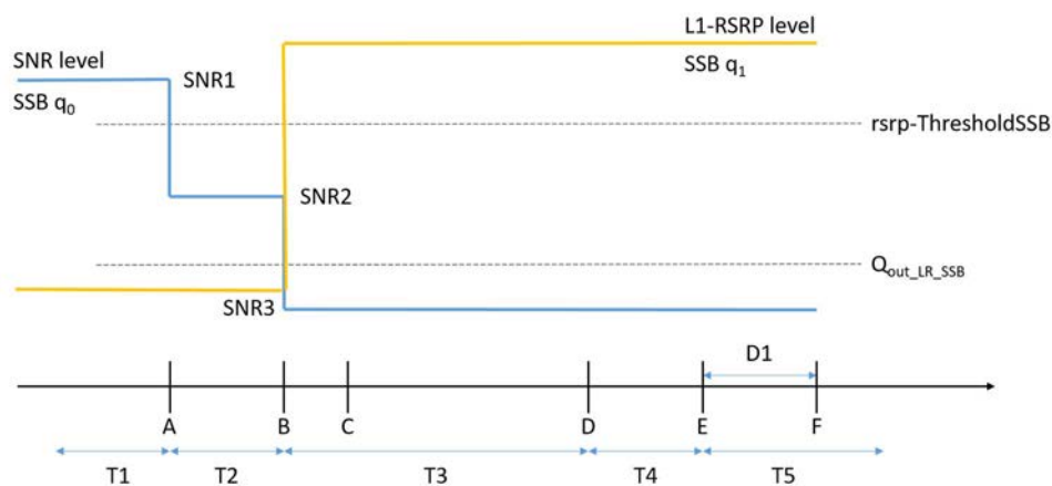
Figure A.11.4.4.1.1-1: SNR and L1-RSRP variation SSB for SSB-based beam failure detection and link recovery testing in non-DRX mode
