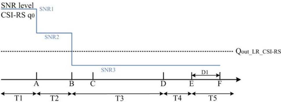
Figure A.5.5.5.7.1-1: SNR variation for CSI-RS-based beam failure detection and link recovery testing for SCell in DRX mode
