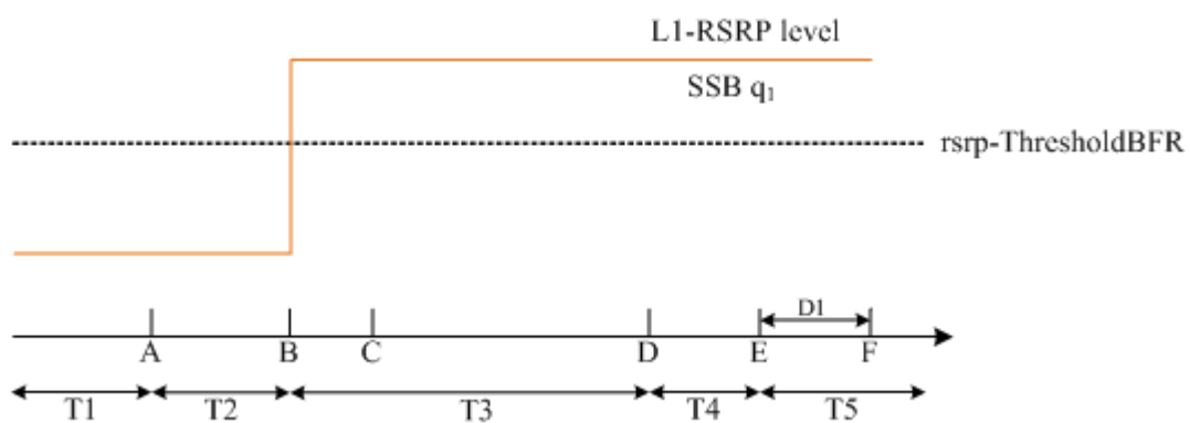
Figure A.4.5.5.6.1-2: L1-RSRP level variation for beam failure detection and link recovery testing for SCell in DRX mode
