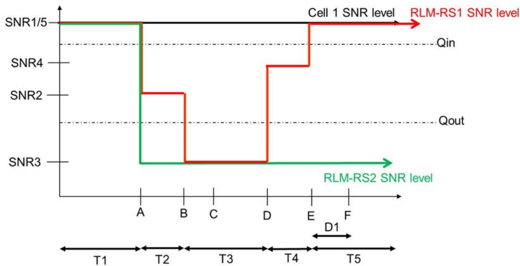
Figure A.5.5.1.8.1-1: SNR variation for CSI-RS in-sync testing
