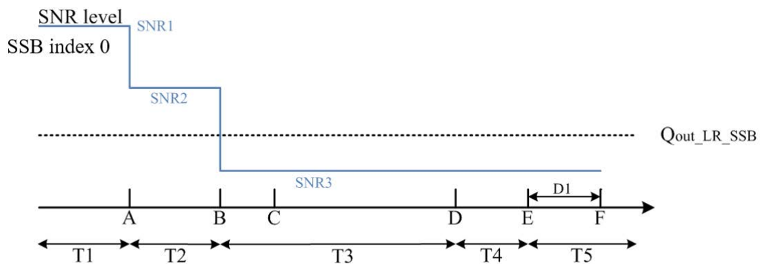
Figure A.5.5.5.1-1: SNR variation for SSB-based beam failure detection and link recovery testing in non-DRX mode
