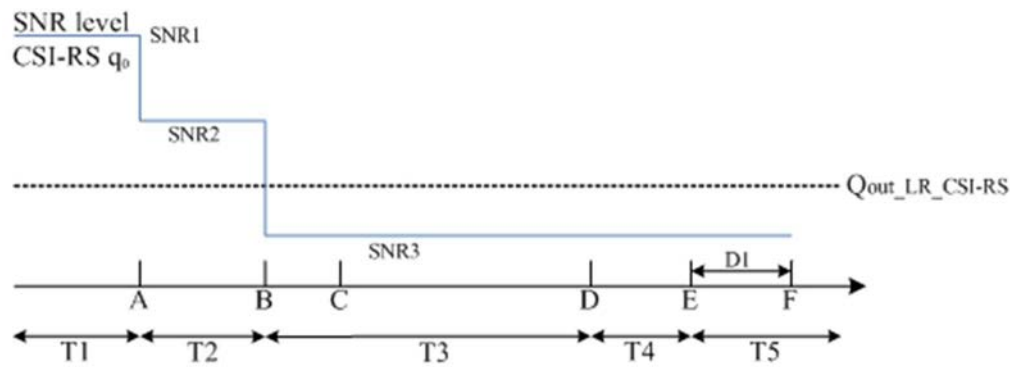
Figure A.6.5.5.1-1: SNR variation for beam failure detection and link recovery testing in for SCell non-DRX mode
