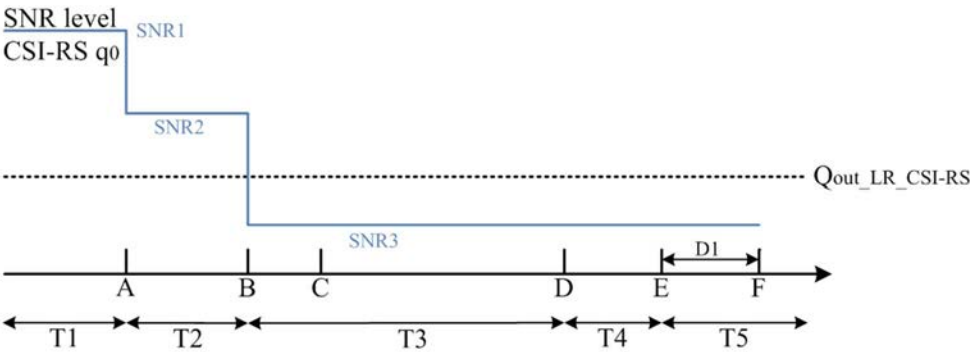
Figure A.5.5.4.1-1: SNR variation for CSI-RS-based beam failure detection and link recovery testing in DRX mode
