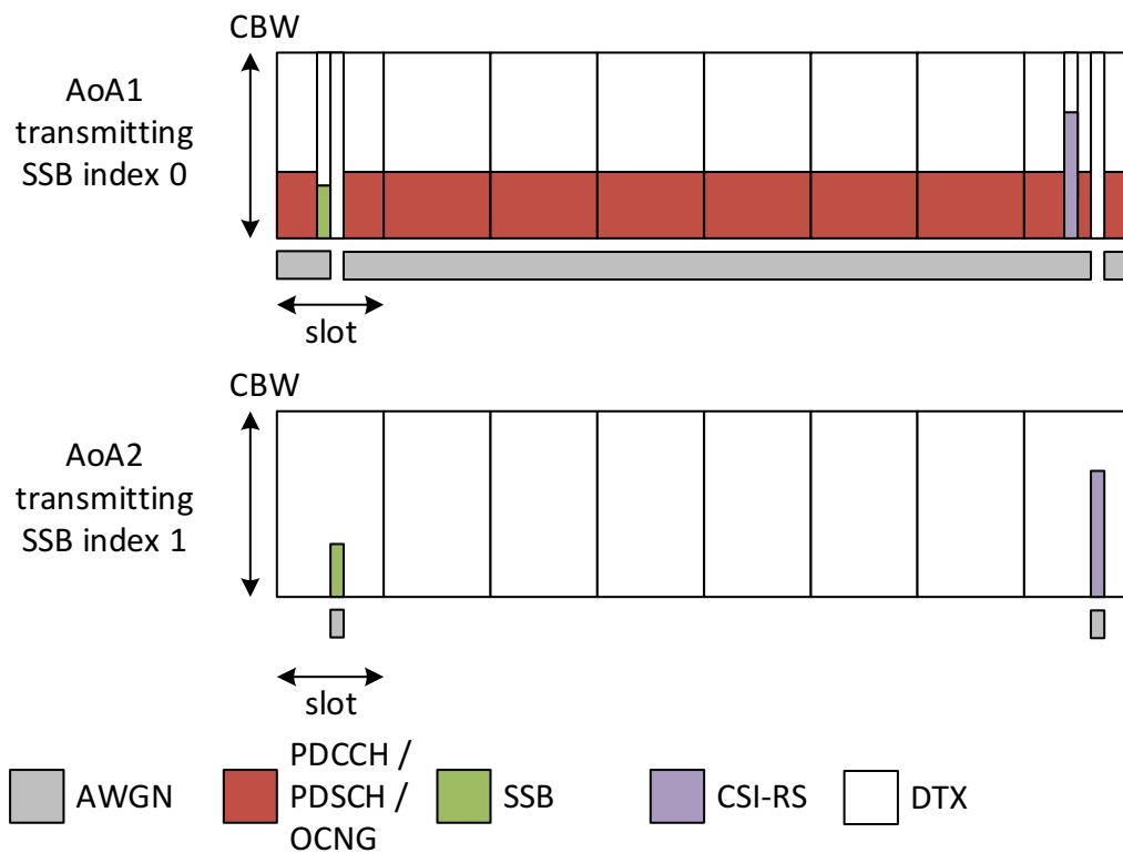
Figure A.7.5.8.2.1.1-1: Time multiplexed downlink transmissions during T1
