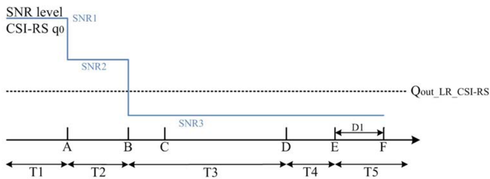
Figure A.7.5.5.6.1-1: SNR variation for beam failure detection and link recovery testing for SCell in non-DRX mode
