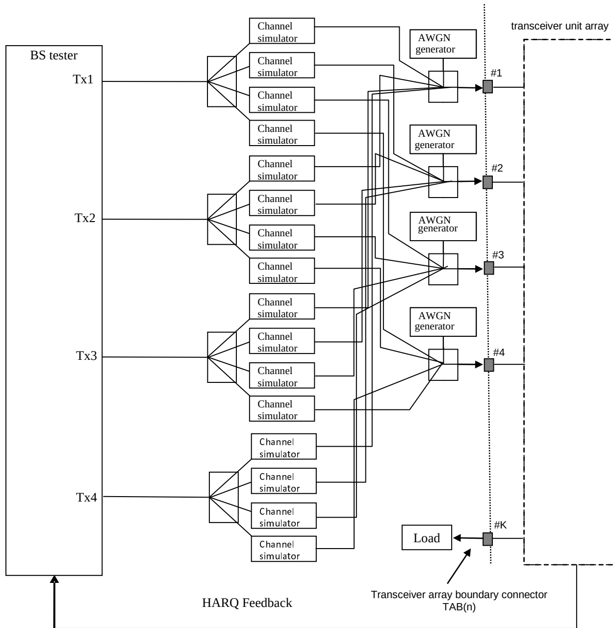
Figure D.6.2A-1: Functional set-up for performance requirements for PUSCH transmission on four antenna ports in multipath fading conditions (4 Rx case shown)
