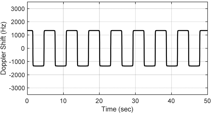
Figure J.3-2: Doppler shift trajectory for scenario 3-NR350 (15 kHz SCS)
