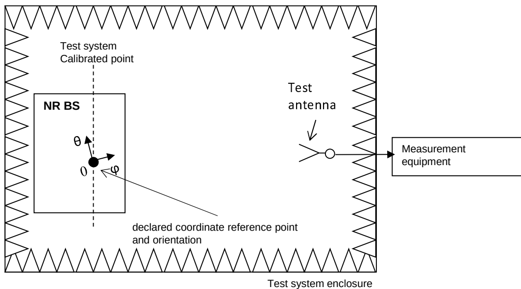
Figure E.1.1-1: Measurement set up for radiated transmit power, OTA output power dynamics, OTA transmitted signal quality, OTA occupied bandwidth, and OTA transmit ON/OFF power ( BS type 2-O )
