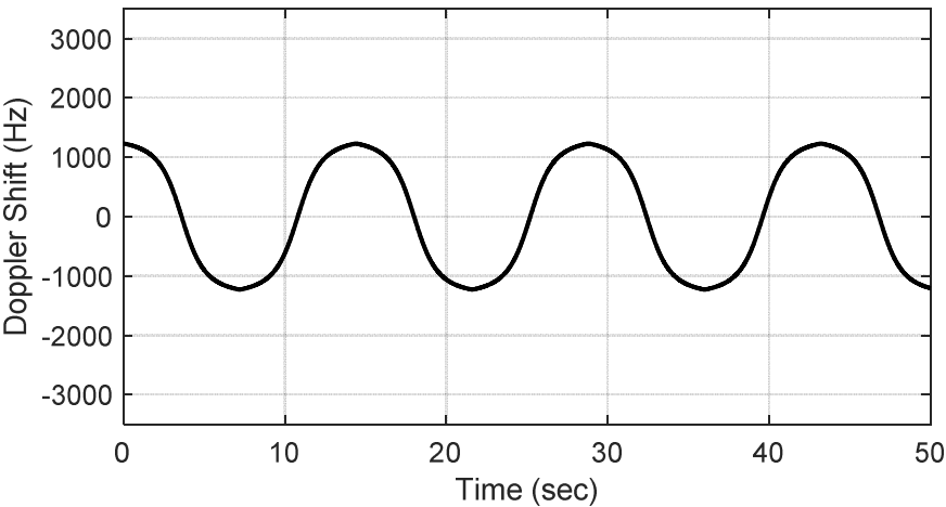
Figure J.3-1: Doppler shift trajectory for scenario 1-NR350 (15 kHz SCS)
