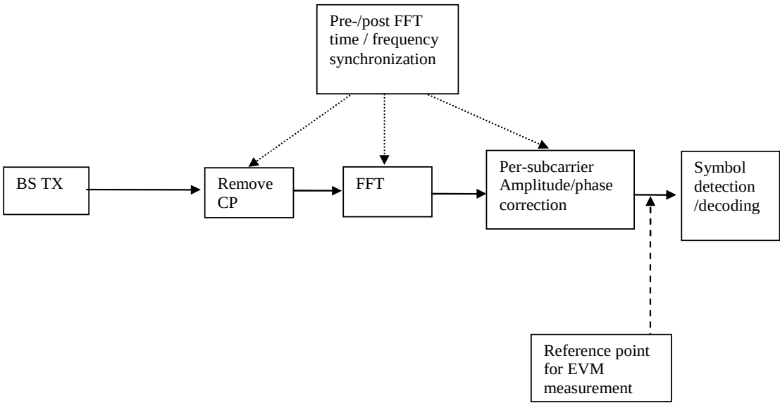
Figure L.2.4-1: Reference point for FR1 EVM measurements
