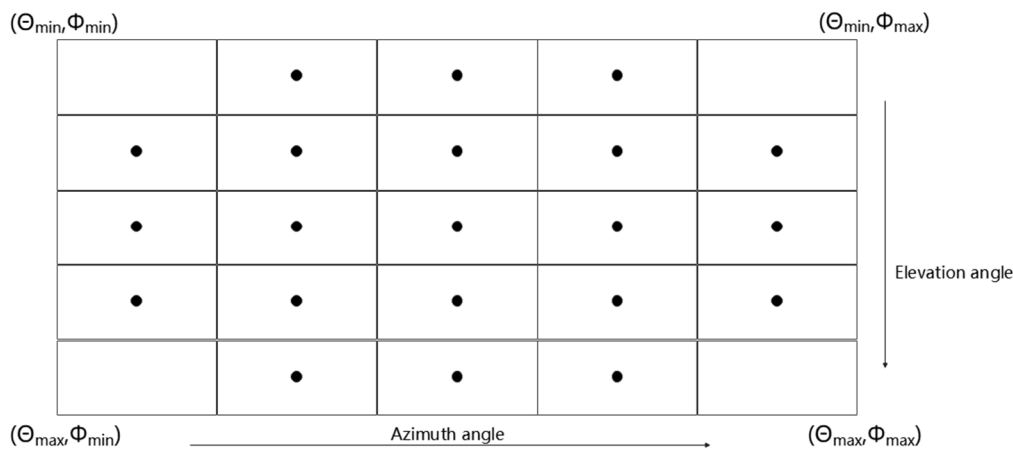
Figure 4.9.3.2-1 Test beam set for conformance testing
