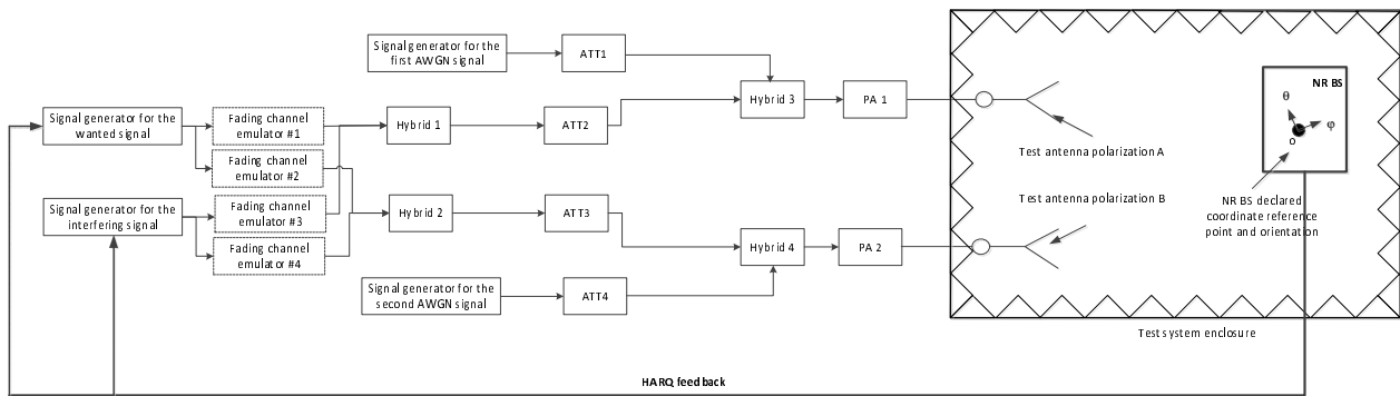
Figure E.3-5: Measurement set up for single TX, dual polarization radiated enhanced performance requirements
