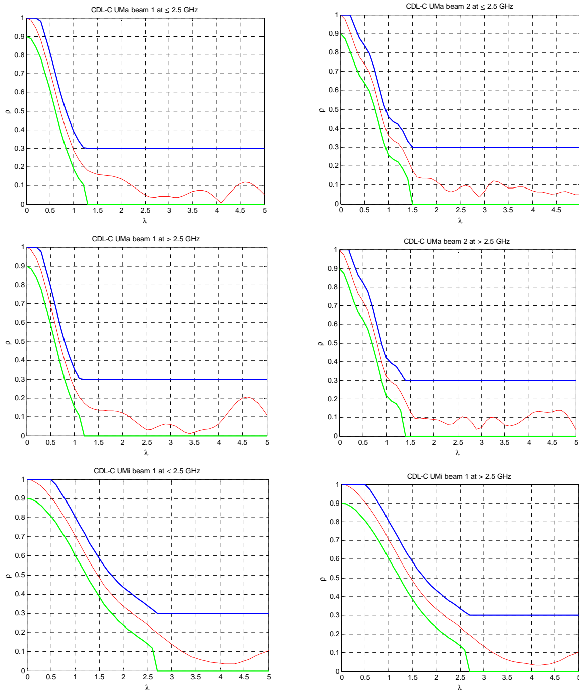
Figure C.4.3-1: Pass/fail limits and targets of Temporal correlation for CDL-C UMa and CDL-C UMi channel model: red curve (reference), blue (upper limit) and green (lower limit)
