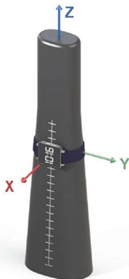
Figure B.3.2.2-1: Positioning guidance for Forearm Phantom in the chamber (© 2001 – 2022 CTIA Certification. Reproduced with permission.), defined in the CTIA Certification OTA Test Plan
