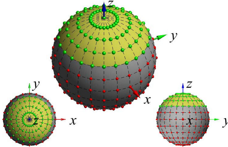
Figure D.2.4.1-1: Visualization of partial surface with \pm 60^\circ angular width for classical TRP grid.
