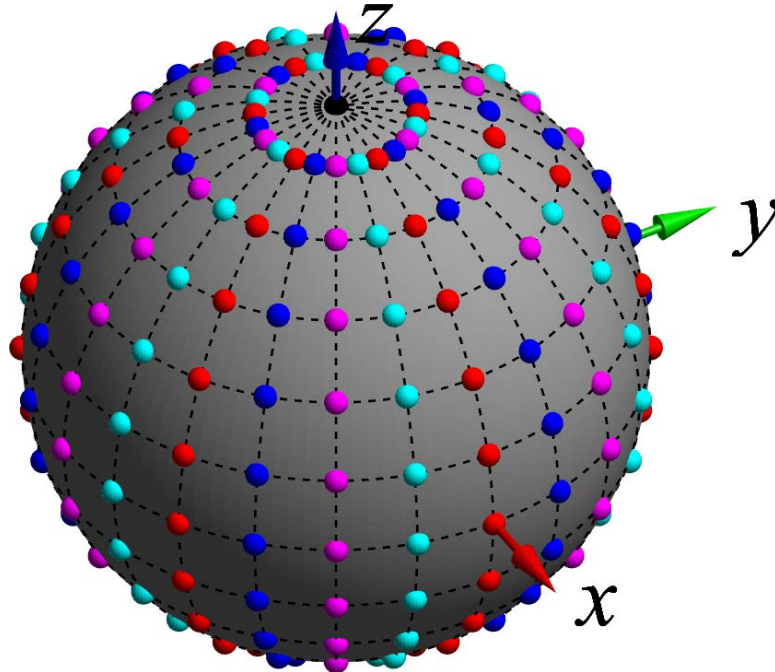
Figure A.3.3.4-1: 266 measurement grid point for TRP.
