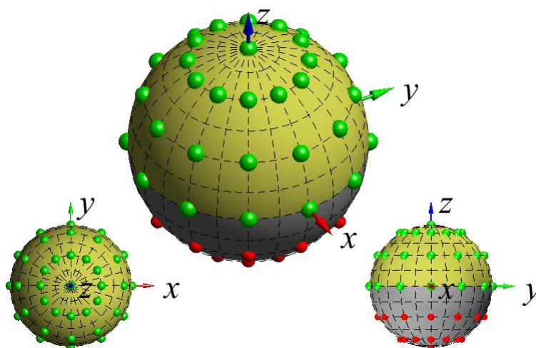
Figure 5.3.1.7-1: Visualization of upper hemisphere partial surface with \pm 90^\circ angular width for classical TRS grids.
