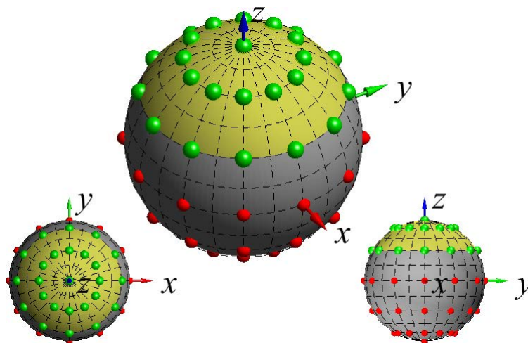
Figure D.2.5.1-1: Visualization of partial surface with \pm 60^\circ angular width for classical TRS grid.
