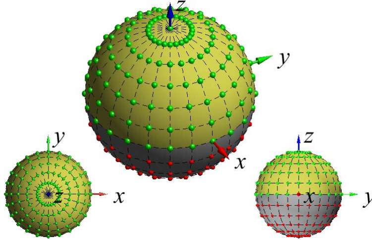
Figure D.2.4.2-1: Visualization of upper hemisphere partial surface with \pm 90^\circ angular width for classical TRP grids.
