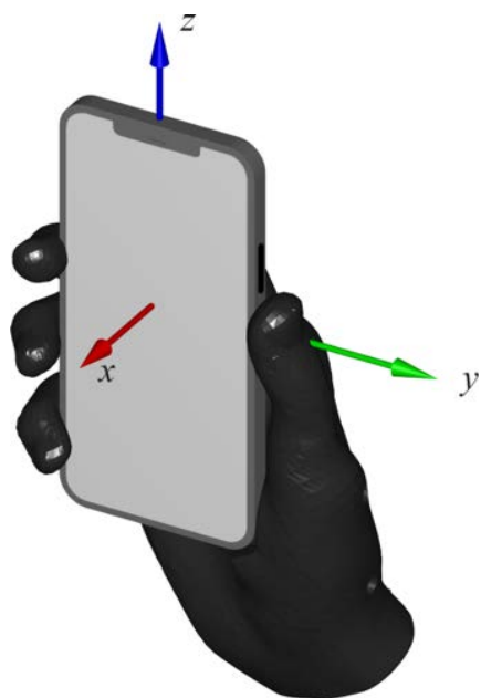
Figure B.3.5-1: Hand phantom only for NTN scenario 2 (default, i.e., elevation tilt 0°)
