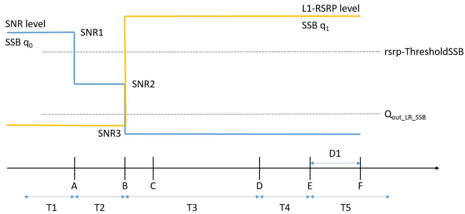
Figure G.2.3B.2.1.1-1: SNR and L1-RSRP variation SSB for SSB-based beam failure detection and link recovery testing
