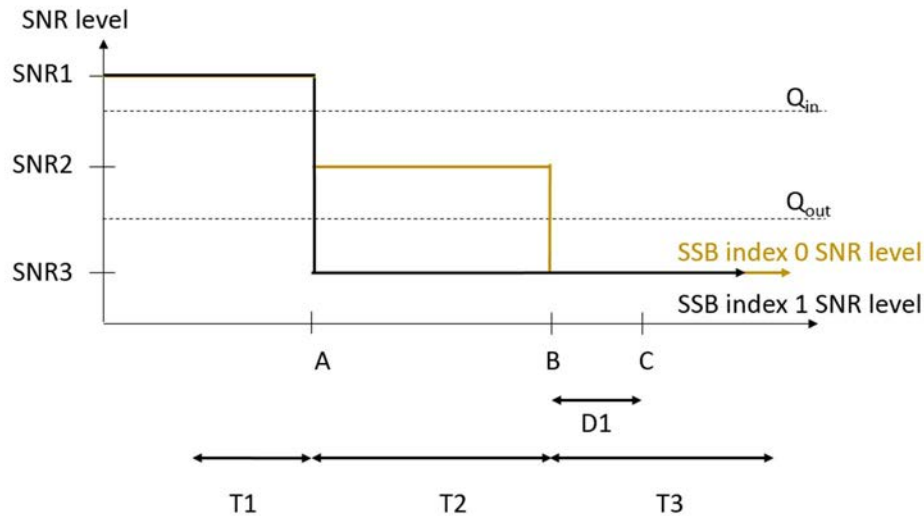
Figure G.2.3B.1.3.1-1: SNR variation for out-of-sync testing
