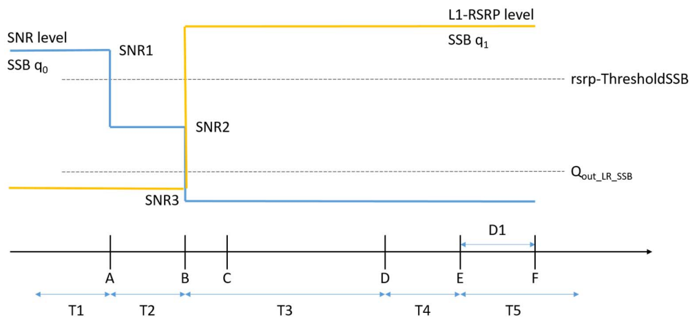
Figure G.2.3B.2.2.1-1: SNR and L1-RSRP variation SSB for SSB-based beam failure detection and link recovery testing in non-DRX mode
