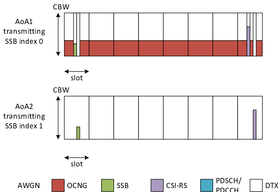
Figure G.2.4B.2.1-1: Time multiplexed downlink transmissions (Config 1 example)
