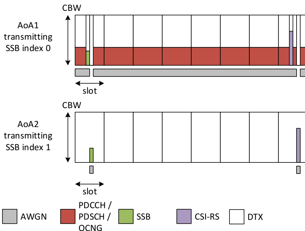
Figure G.2.3B.3.2.1.1-1: Time multiplexed downlink transmissions during T1
