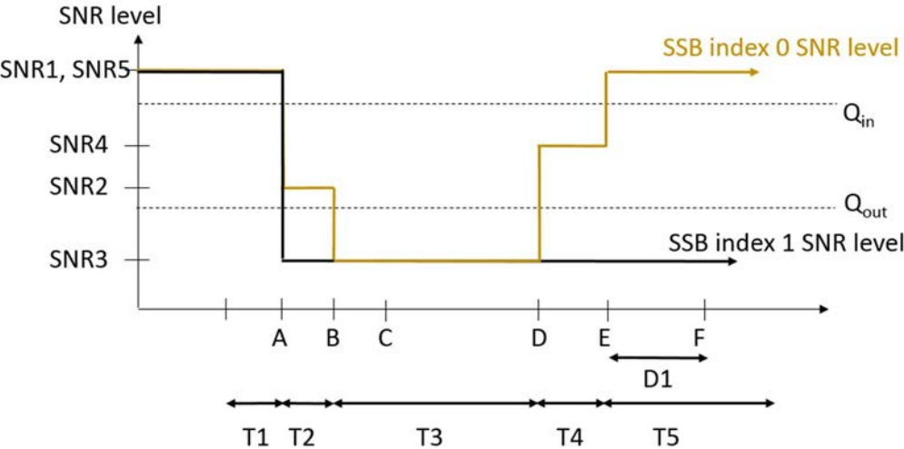
Figure G.2.3B.1.4.1-1: SNR variation for in-sync testing
