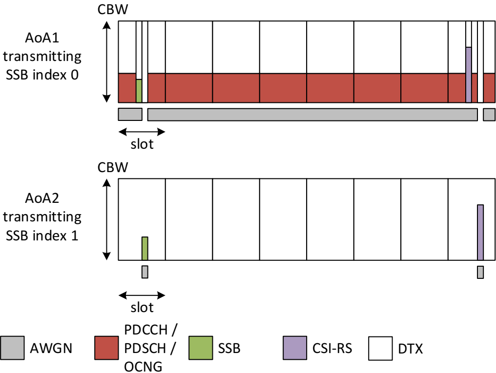
Figure G.2.3B.3.1.1.1-1: Time multiplexed downlink transmissions during T1
