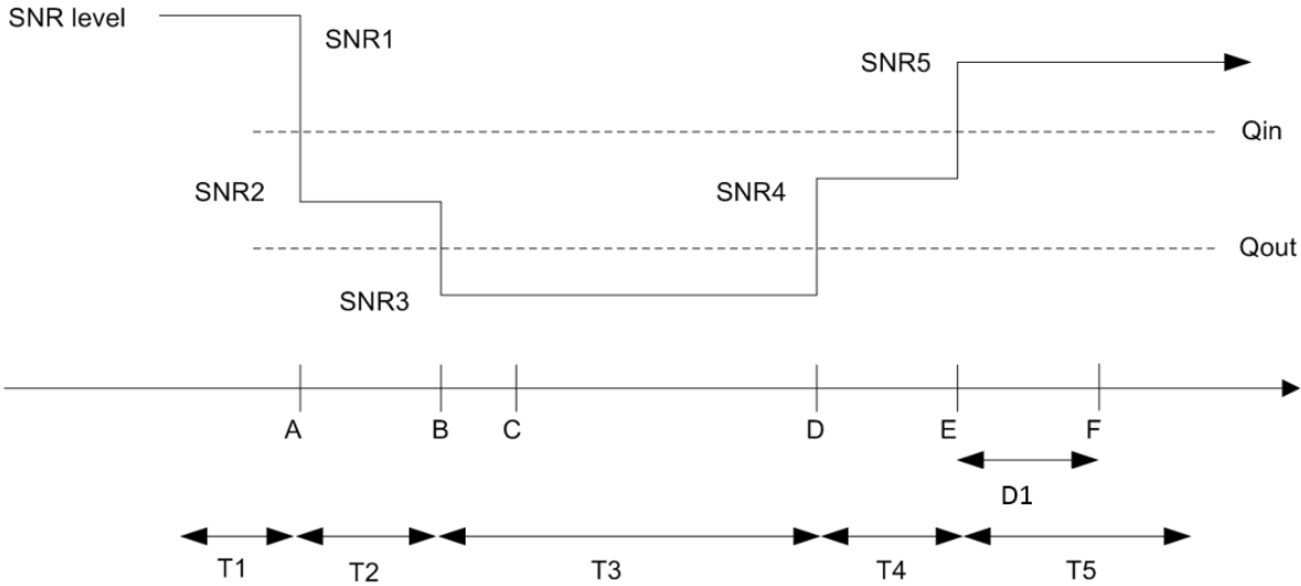
Figure G.2.3B.1.2.1-1: SNR variation for in-sync testing
