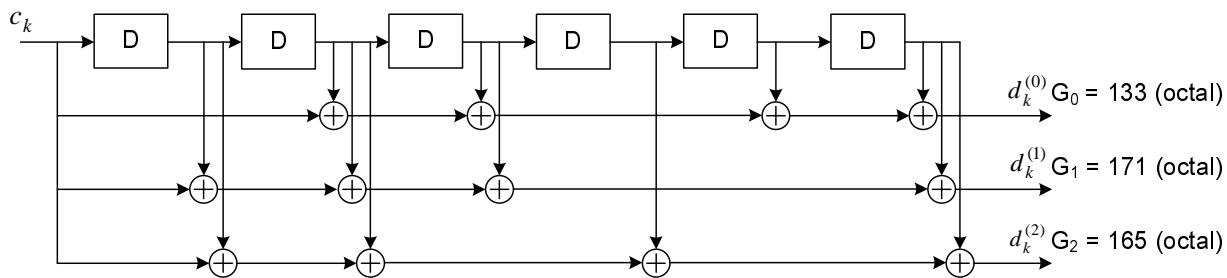
Figure 8.2-1: Rate 1/3 tail biting convolutional encoder
