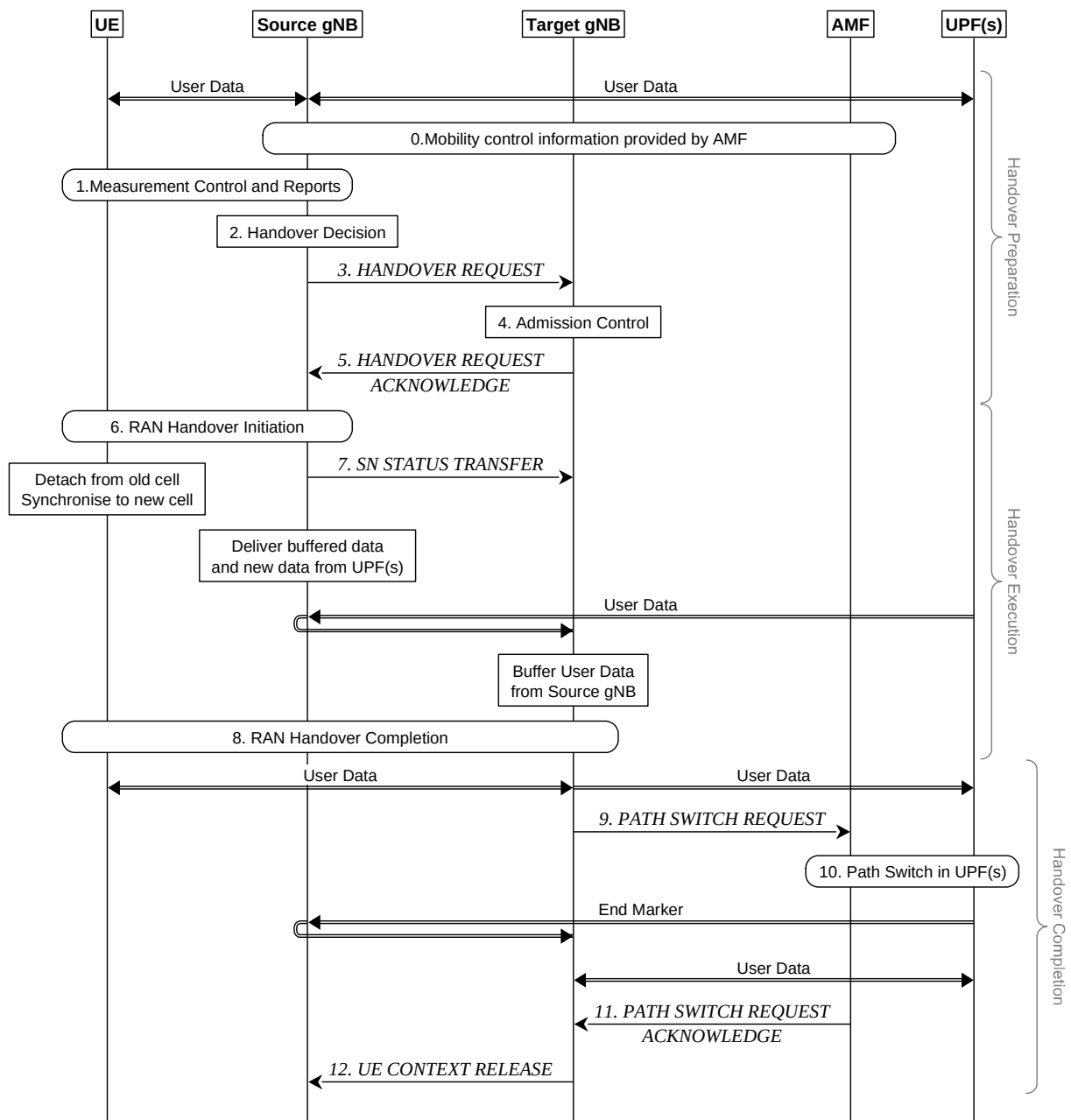
Figure 9.2.3.2.1-1: Intra-AMF/UPF Handover
