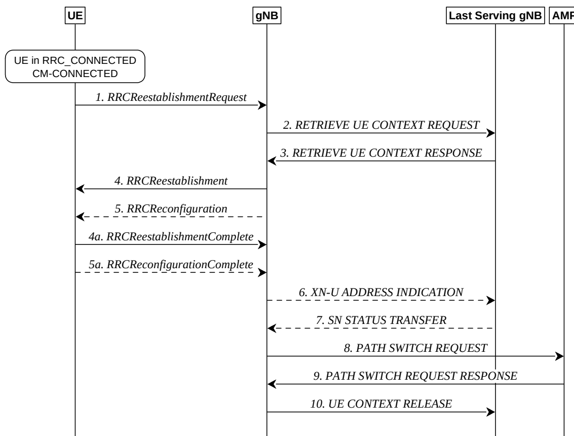
Figure 9.2.3.3-1: Re-establishment procedure
