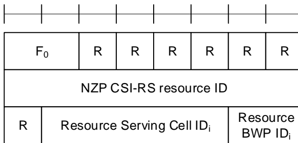
Figure 6.1.36-2: Spatial Relation for Resource ID i with NZP CSI-RS
