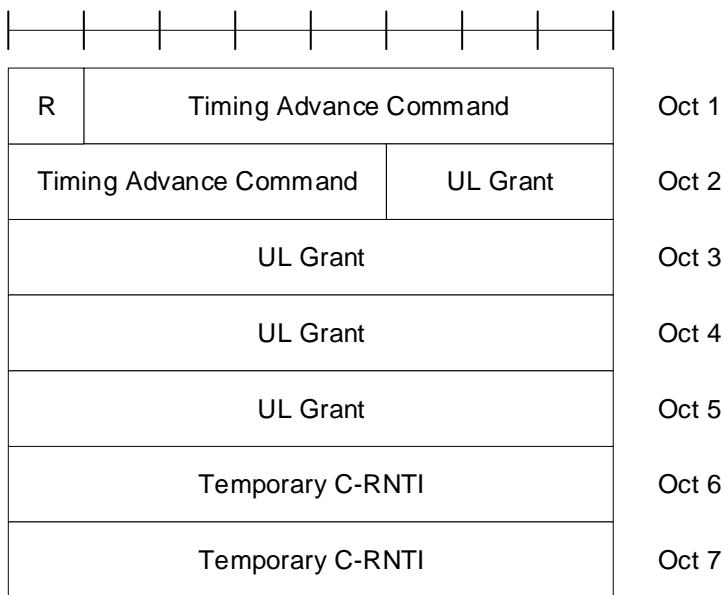
Figure 6.2.3a-1: fallbackRAR
