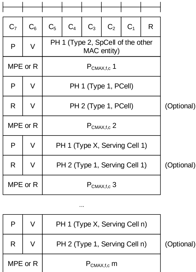
Figure 6.1.3.51-1: Enhanced Multiple Entry PHR for multiple TRP MAC CE with the highest ServCellIndex of Serving Cell with configured uplink is less than 8
