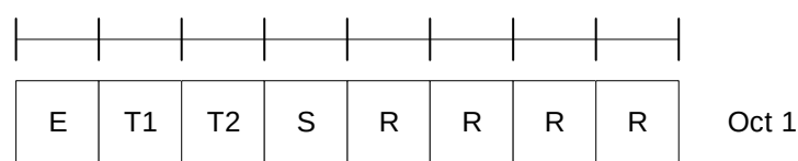
Figure 6.1.5a-3: SuccessRAR MAC subheader
