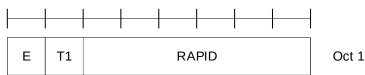
Figure 6.1.5a-2: FallbackRAR MAC subheader
