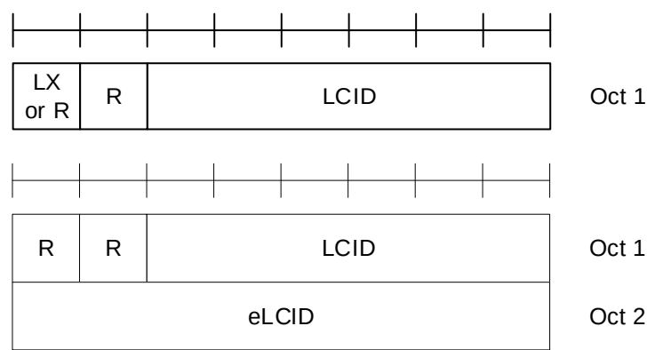
Figure 6.1.2-3: (LX)/R/LCID/(eLCID) MAC subheader
