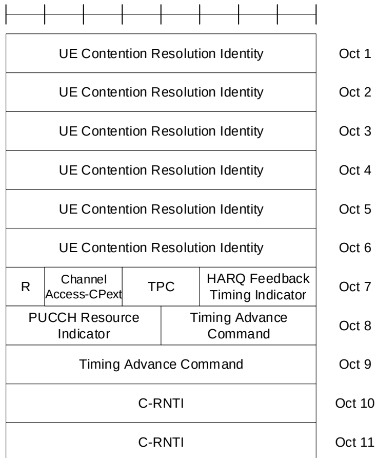
Figure 6.2.3a-2: successRAR
