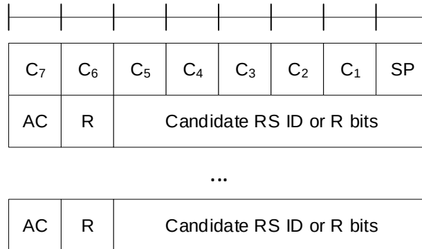
Figure 6.1.3.23-1: BFR and Truncated BFR MAC CE with one octet C i field
