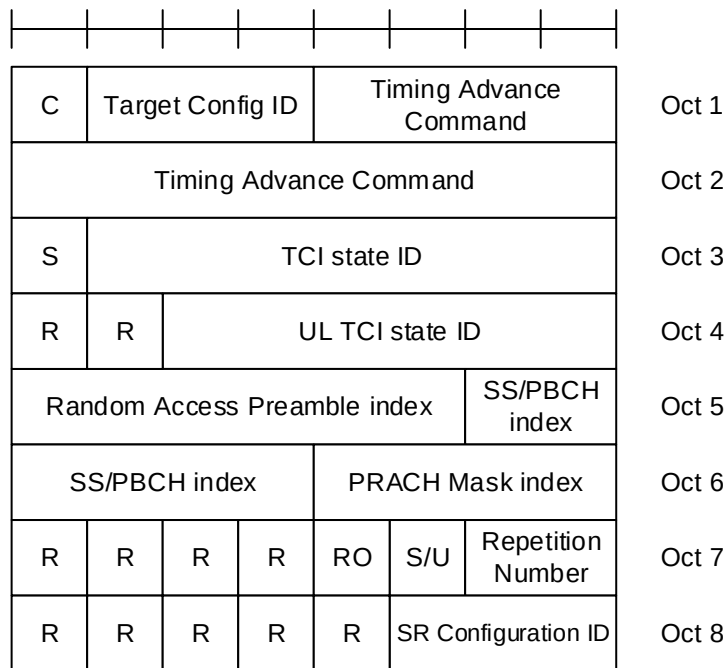
Figure 6.1.3.75-1: LTM Cell Switch Command MAC CE
