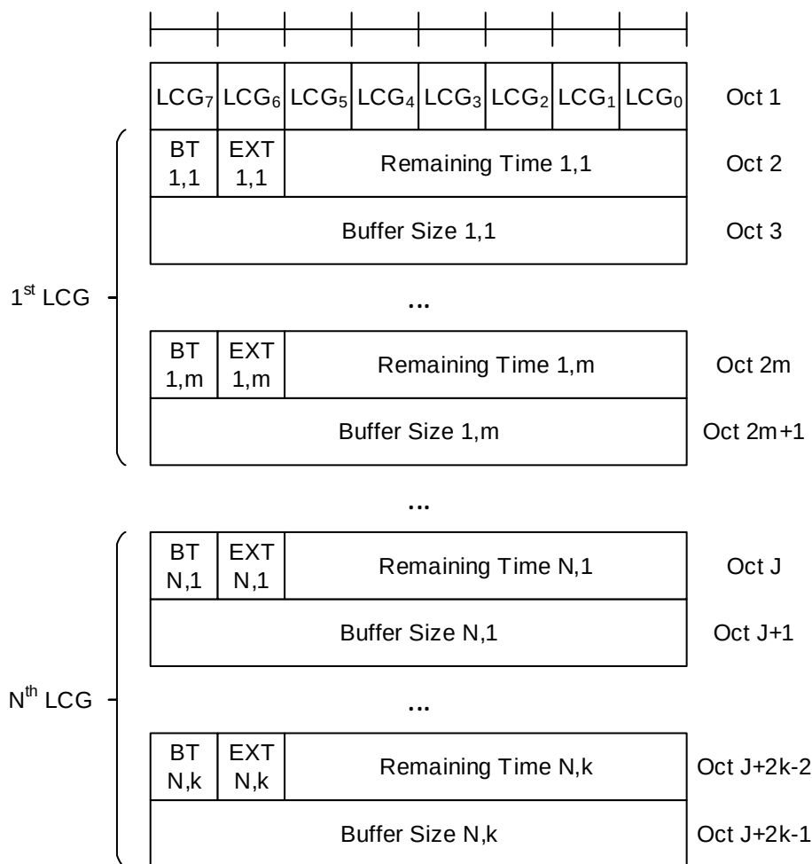
Figure 6.1.3.72-2 Multiple Entry DSR MAC CE
