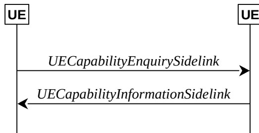
Figure 5.8.9.2.1-1: Sidelink UE capability transfer
