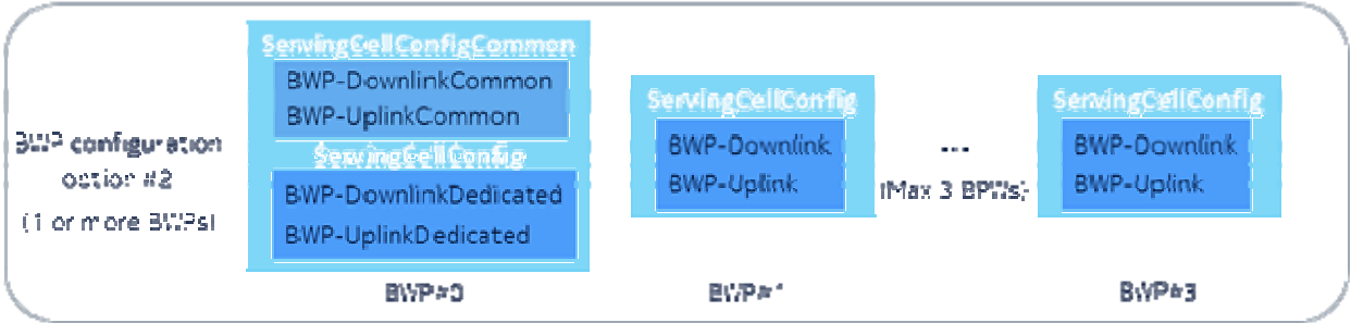
Figure B2-2: BWP#0 configuration with dedicated configuration
