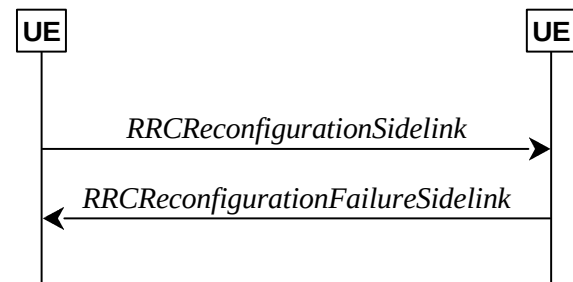
Figure 5.8.9.1.1-2: Sidelink RRC reconfiguration, failure
