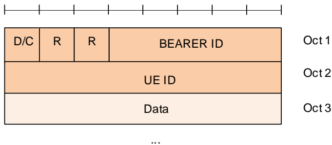
Figure 6.2.2-1: U2N SRAP Data PDU format with SRAP header
