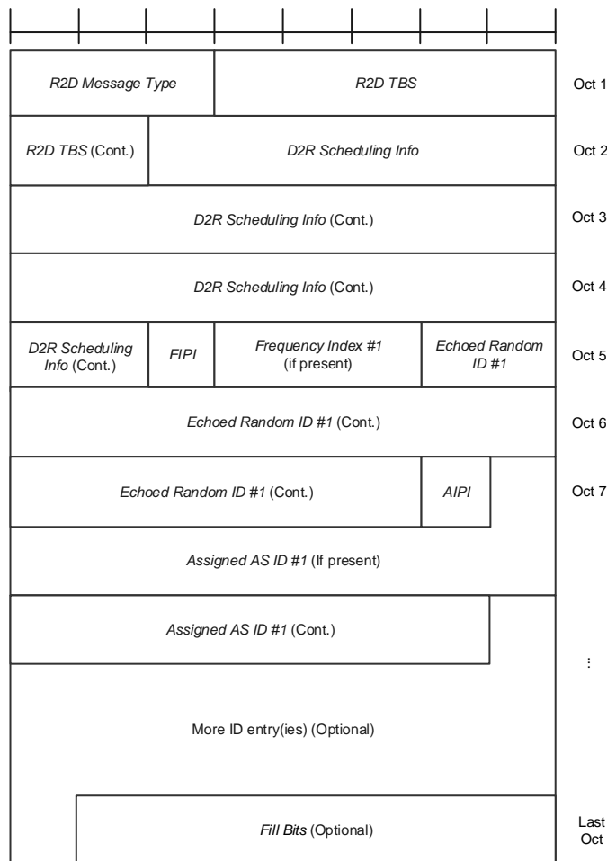
Figure 6.2.1.3-1: MAC PDU of Random ID Response message
