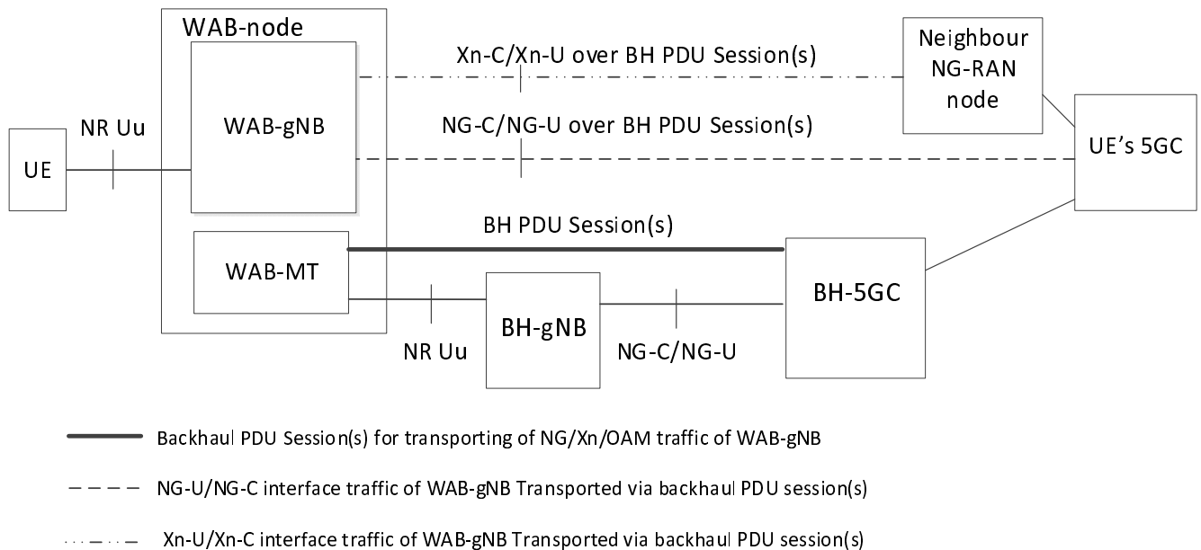
Figure 6.1.7-1: The WAB architecture
