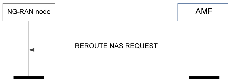
Figure 8.6.5.2-1: Reroute NAS request
