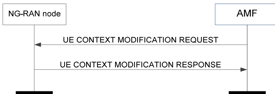
Figure 8.3.4.2-1: UE context modification: successful operation
