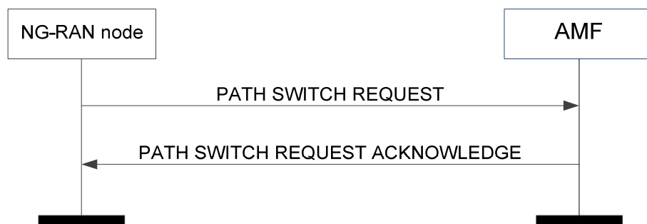
Figure 8.4.4.2-1: Path switch request: successful operation
