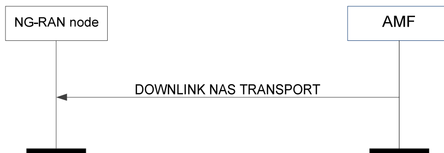
Figure 8.6.2.2-1: Downlink NAS transport
