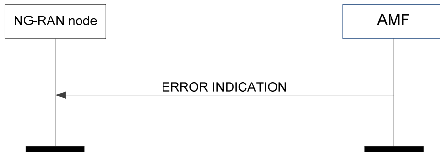
Figure 8.7.5.2-1: Error indication initiated by the AMF
