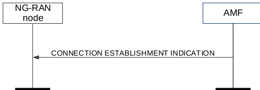
Figure 8.3.6.2-1: Connection Establishment Indication procedure. Successful operation.
