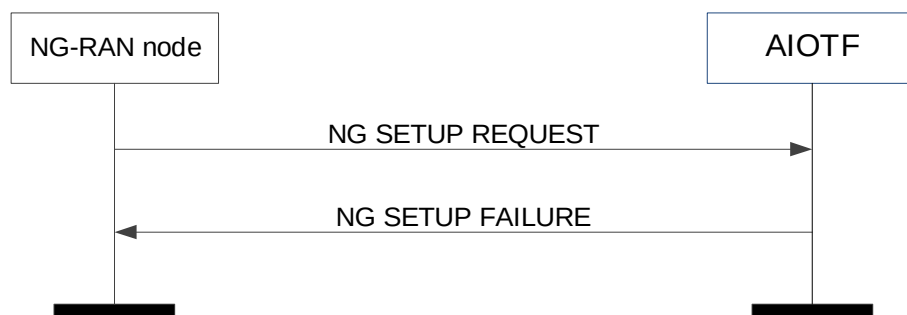
Figure 8.7.1.3-2: NG setup: unsuccessful operation with the AIOTF
