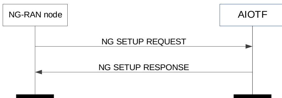
Figure 8.7.1.2-2: NG setup: successful operation with the AIOTF
