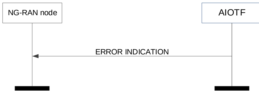
Figure 8.7.5.2-3: Error indication initiated by the AIOTF
