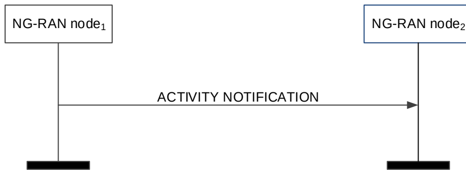
Figure 8.3.11.2-1: Activity Notification
