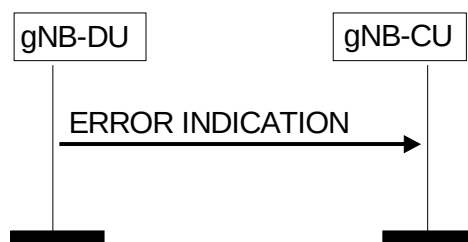
Figure 8.2.2.2-2: Error Indication procedure, gNB-DU originated. Successful operation
