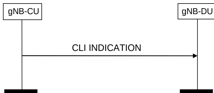
Figure 8.2.15.2-2: CLI Indication initiated from the gNB-CU, successful operation
