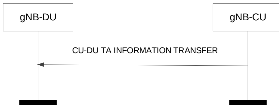
Figure 8.2.13.2-1: CU-DU TA Information Transfer procedure. Successful operation.
