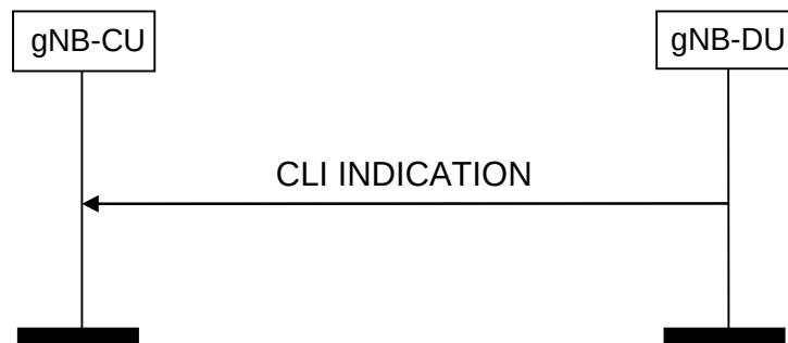
Figure 8.2.15.2-1: CLI Indication initiated from the gNB-DU, successful operation
