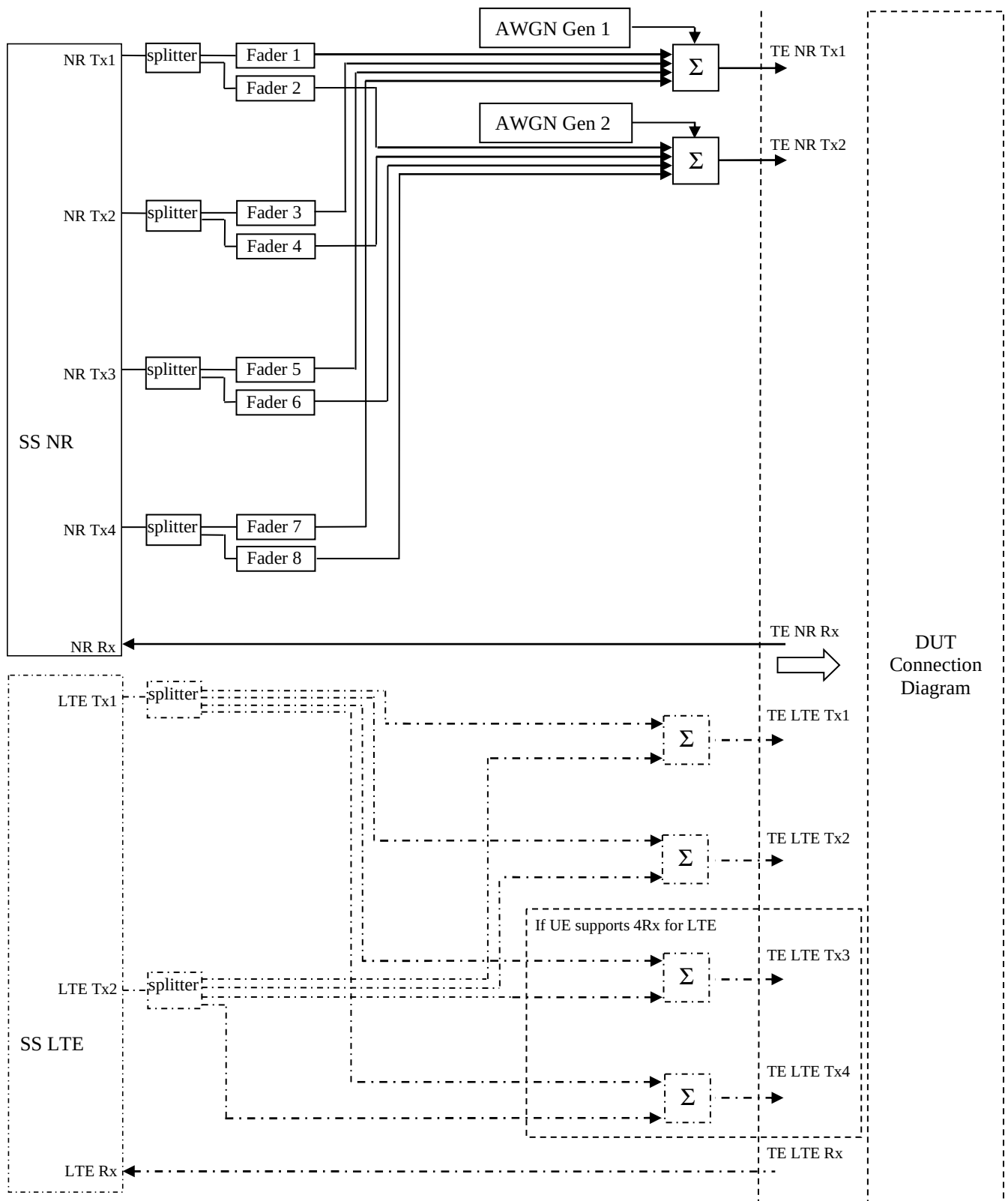
Figure A.3.1.7.8: Test Equipment connection for Demodulation Performance and CSI reporting tests with antenna configuration 4x2
