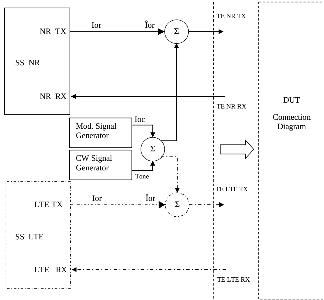
Figure A.3.1.4.3: Test Equipment connection for Receiver tests both Modulated and additional CW Interference signal
