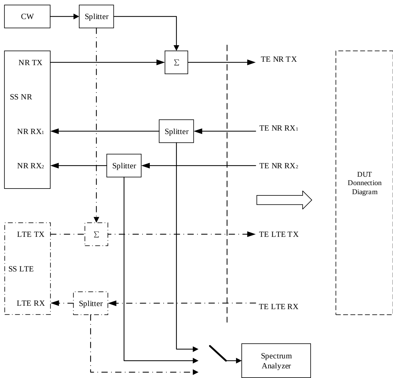
Figure A.3.1.3.2: Test Equipment connection for Transmitter tests for 2Tx UL MIMO or NR 2Tx Tx diversity with CW Interference and spectrum analyser
