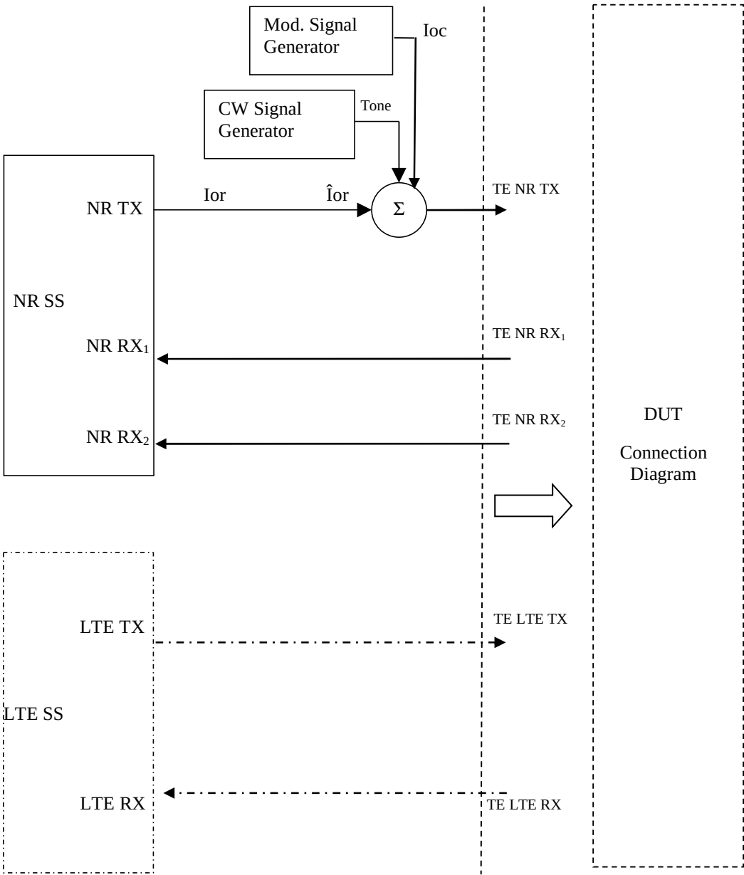
Figure A.3.1.4.6: Test Equipment connection for Receiver tests for 2Tx UL MIMO or NR 2Tx Tx diversity with both Modulated and additional CW Interference signal
