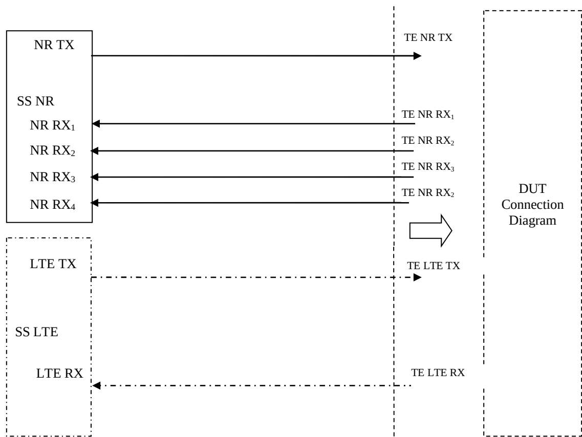
Figure A.3.1.1.2a: Test Equipment connection for single cell, RX and TX tests for NR 4Tx UL MIMO or NR 4Tx Tx diversity
