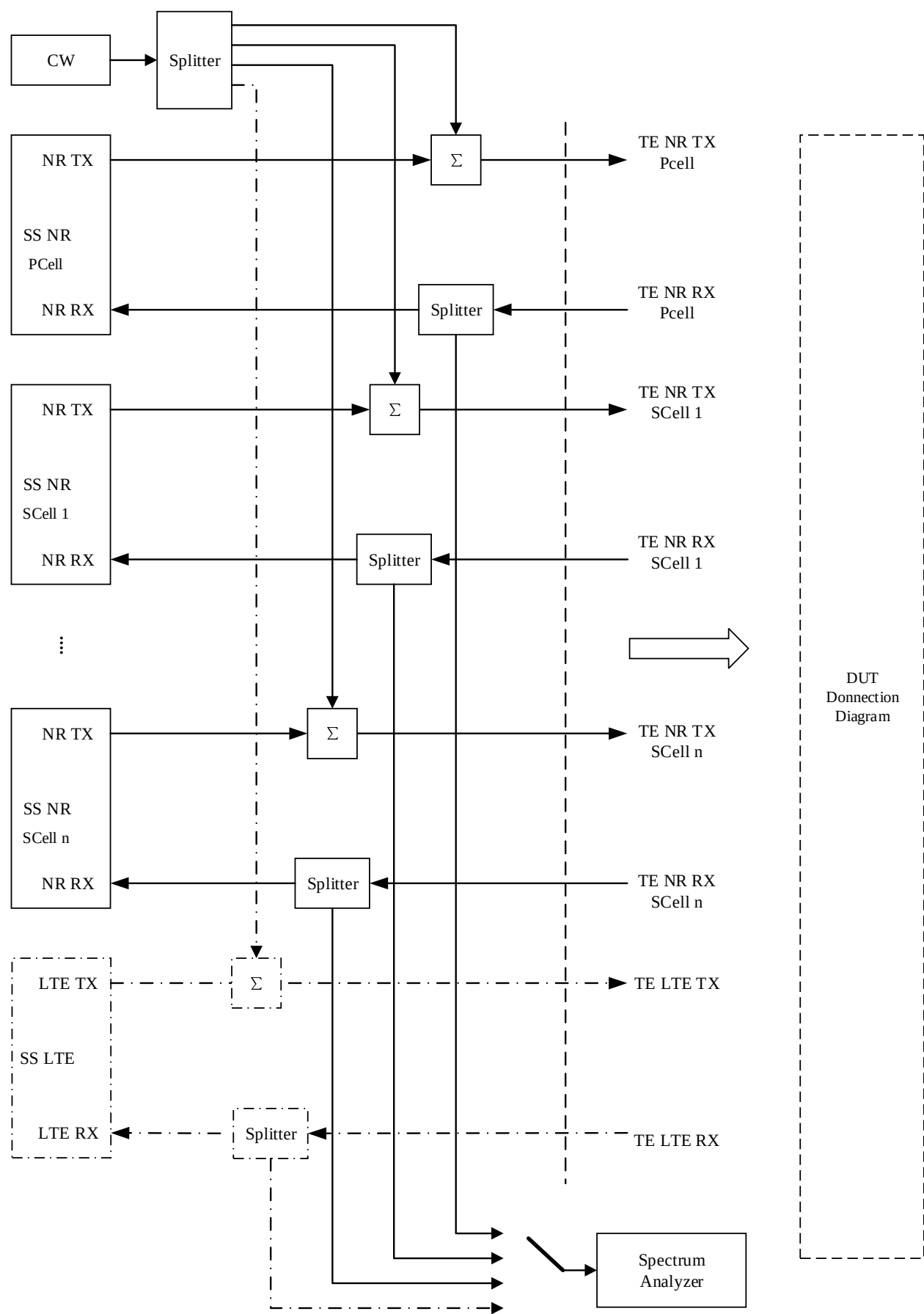
Figure A.3.1.3.3: Test Equipment connection for NR CA Transmitter tests with CW Interference and spectrum analyzer
