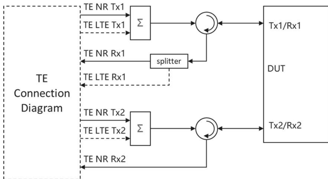
Figure A.3.2.3.4a: 2 Tx User Equipment connection for tests with more than one cell with NR and LTE cells at the same connectors for both cells and 2TX UL MIMO or Tx diversity supported
