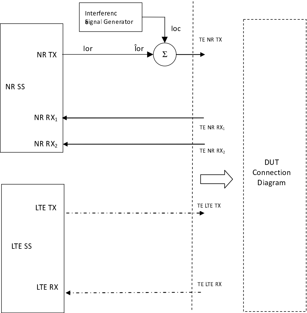
Figure A.3.1.4.4: Test Equipment connection for Receiver tests for 2Tx UL MIMO or NR 2Tx Tx diversity with Modulated Interference
