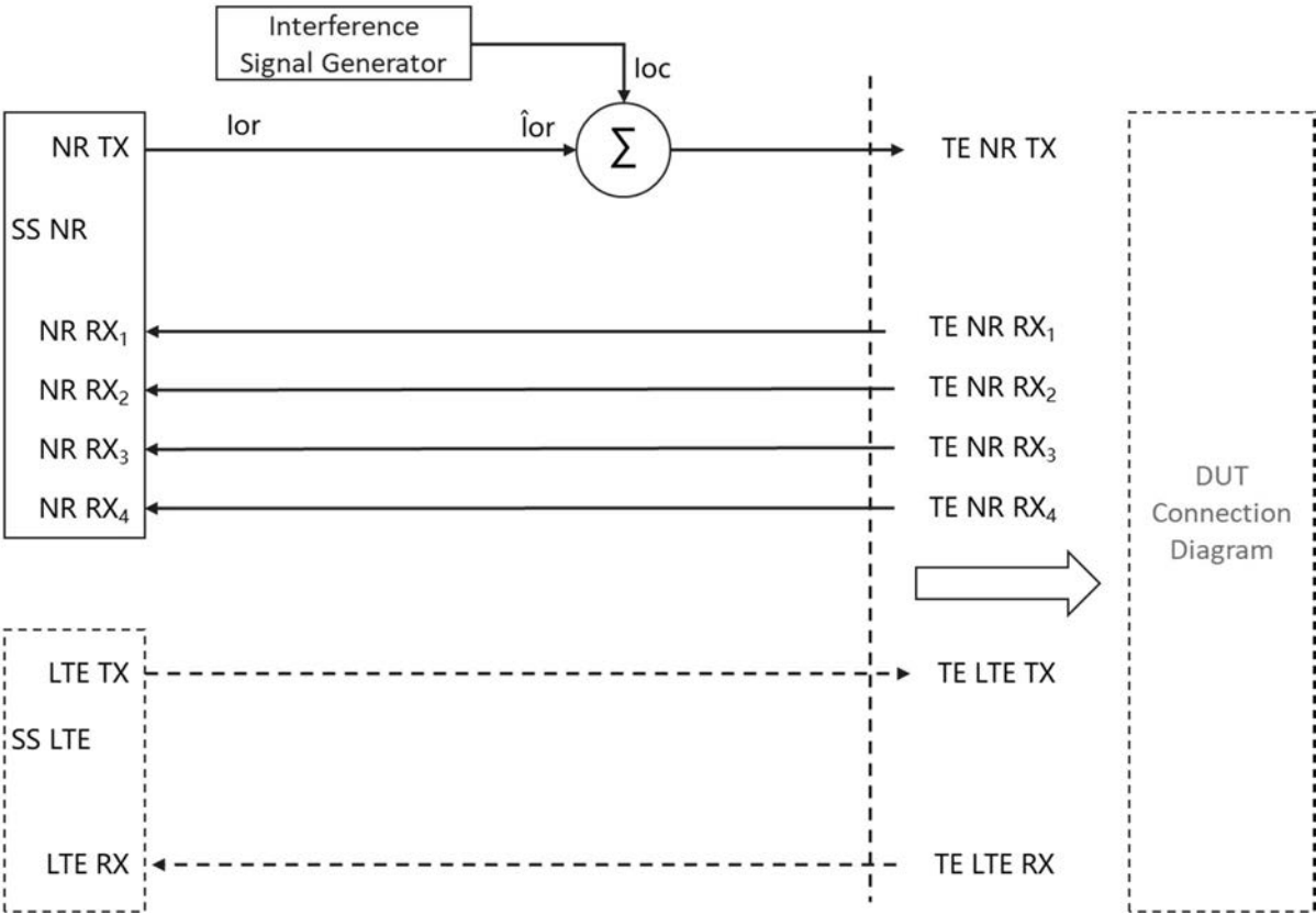
Figure A.3.1.4.4a: Test Equipment connection for Receiver tests for NR 4Tx UL MIMO or NR 4Tx Tx diversity with Modulated Interference
