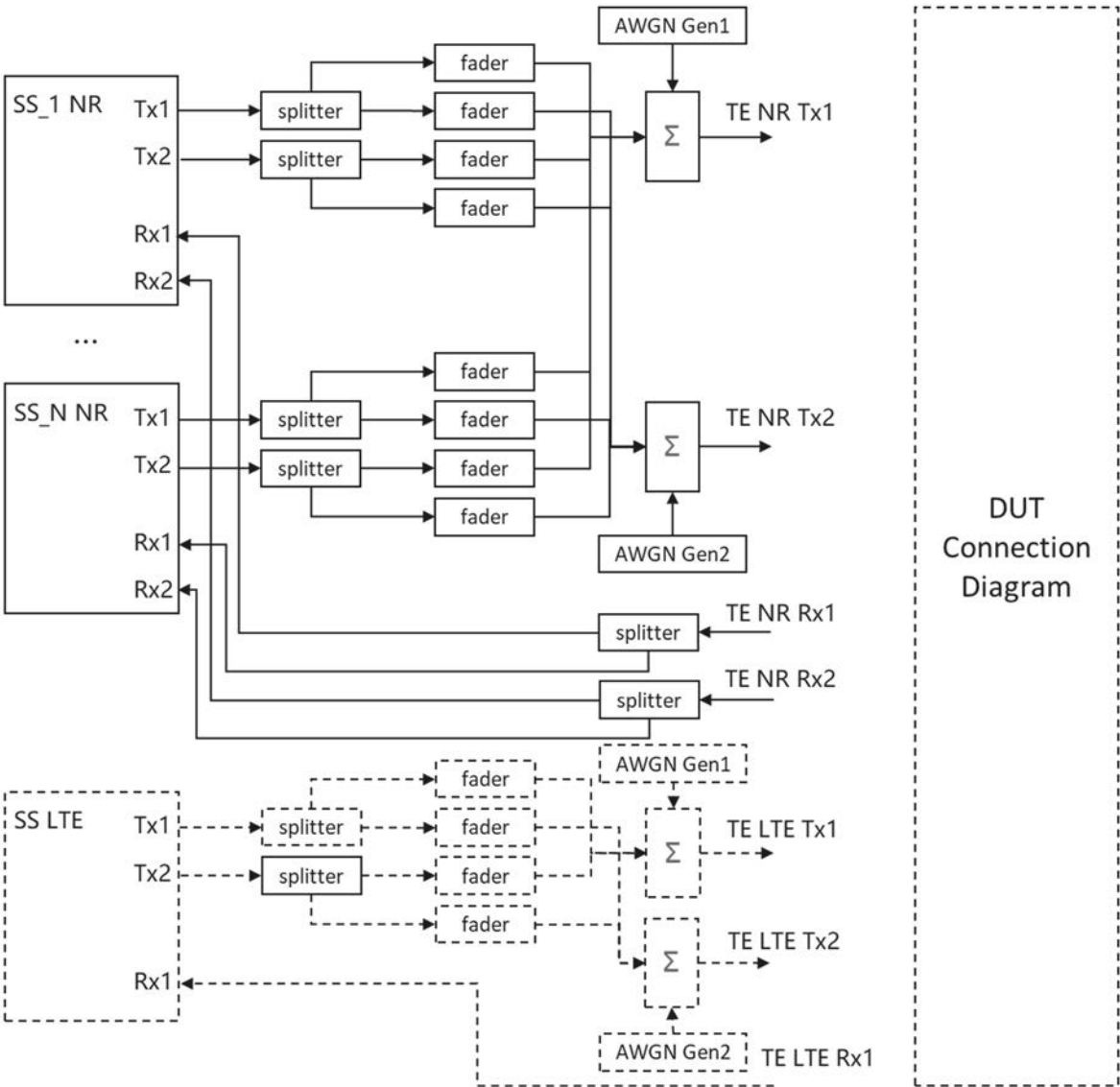
Figure A.3.1.8.2b: Test Equipment connection for UL MIMO tests with more than one NR cell and antenna configuration 2x2
