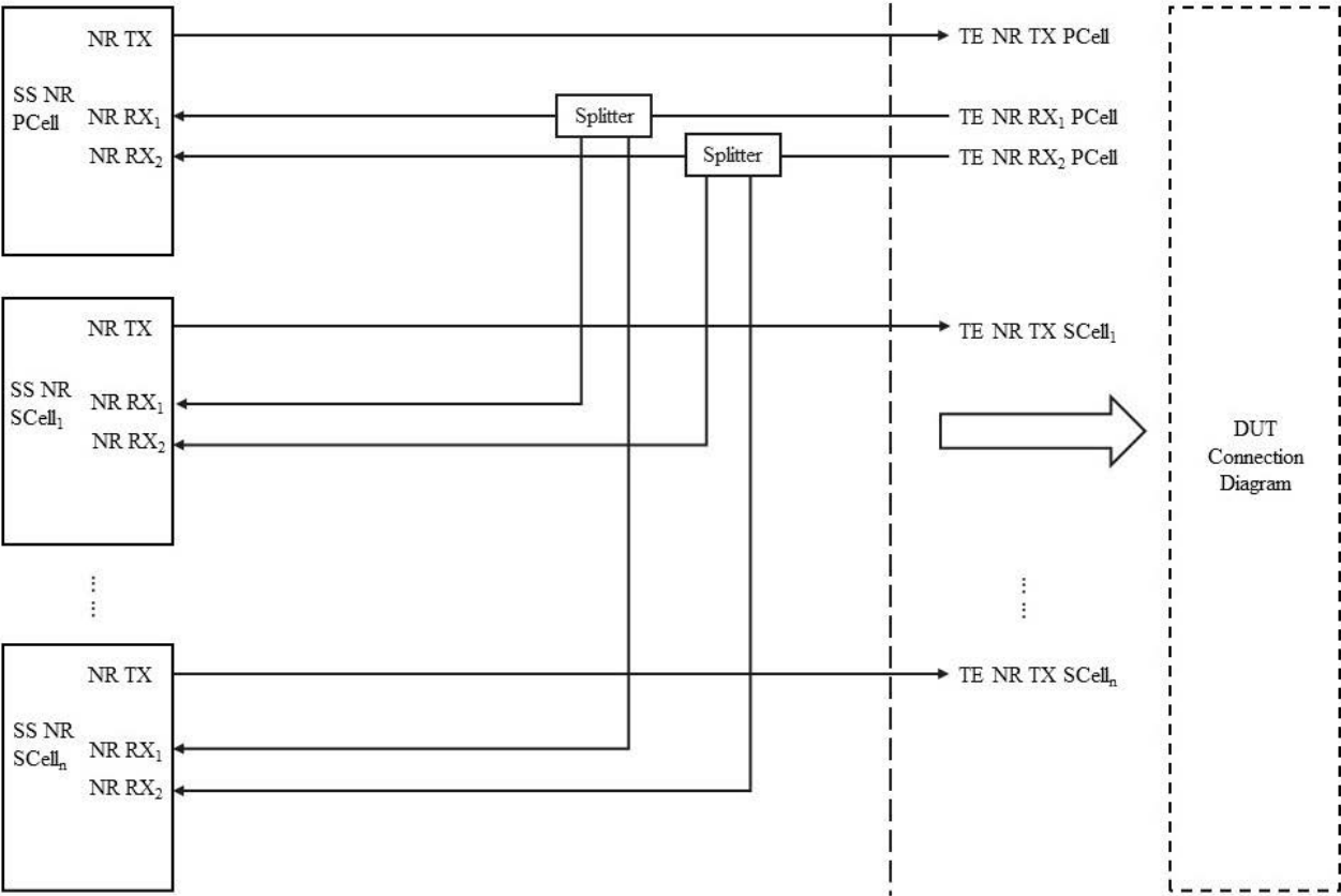
Figure A.3.1.1.9: Test Equipment connection for inter-band UL CA for UL Tx Switching
