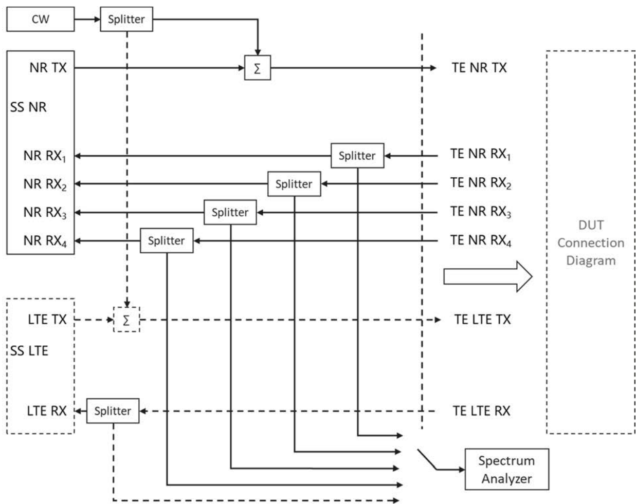
Figure A.3.1.3.2a: Test Equipment connection for Transmitter tests for NR 4Tx UL MIMO or NR 4Tx Tx diversity with CW Interference and spectrum analyser
