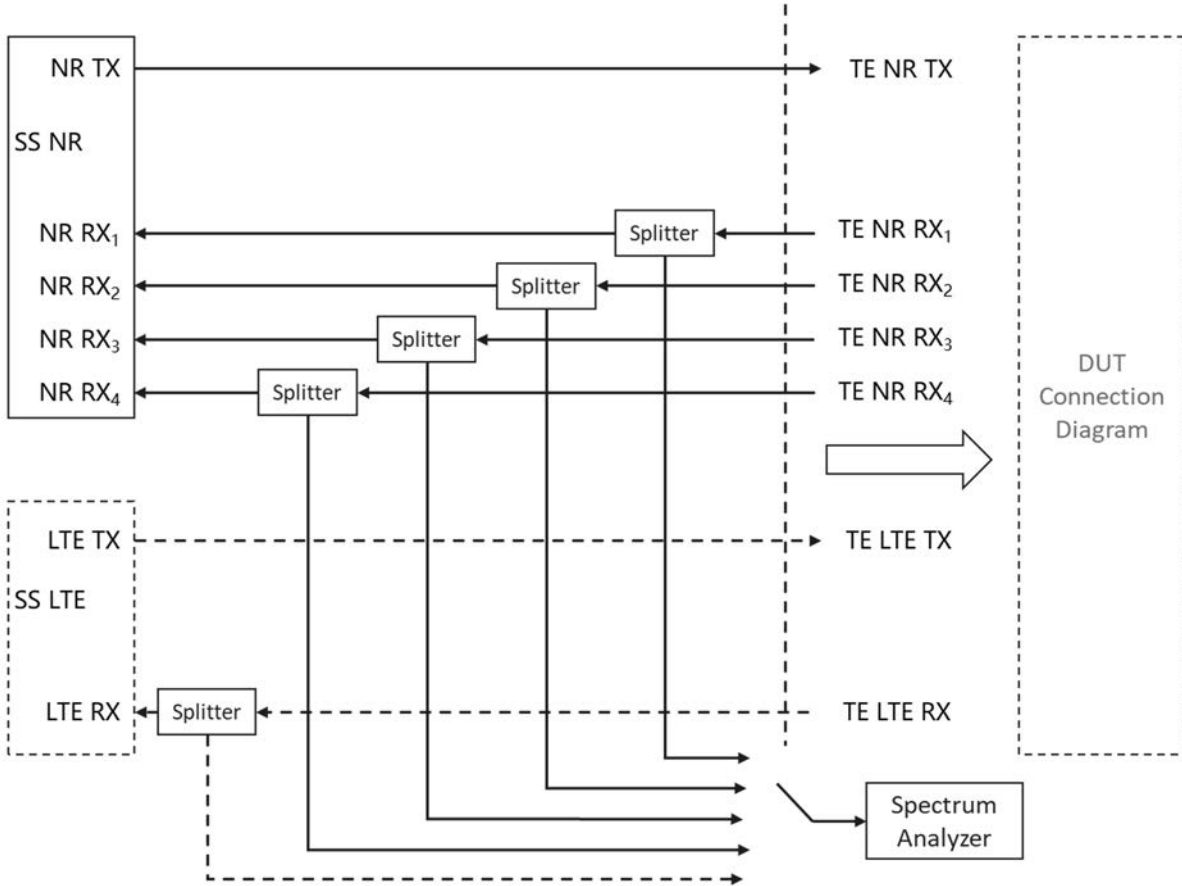
Figure A.3.1.2.2a: Test Equipment connection for TX-tests for NR 4Tx UL MIMO or NR 4Tx Tx diversity with additional Spectrum Analyser
