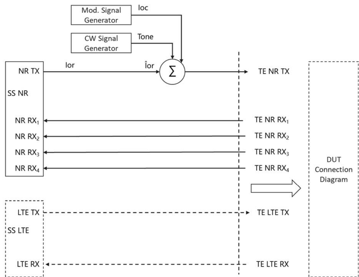
Figure A.3.1.4.6a: Test Equipment connection for Receiver tests for NR 4Tx UL MIMO or NR 4Tx Tx diversity with both Modulated and additional CW Interference signal
