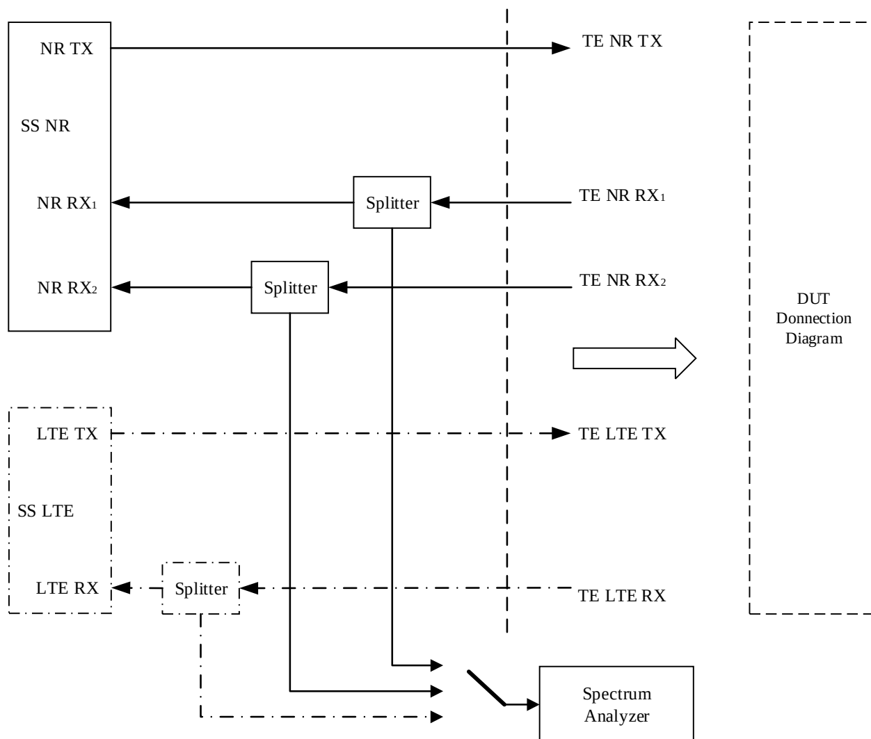
Figure A.3.1.2.2: Test Equipment connection for TX-tests for 2Tx UL MIMO or NR 2Tx Tx diversity with additional Spectrum Analyser
