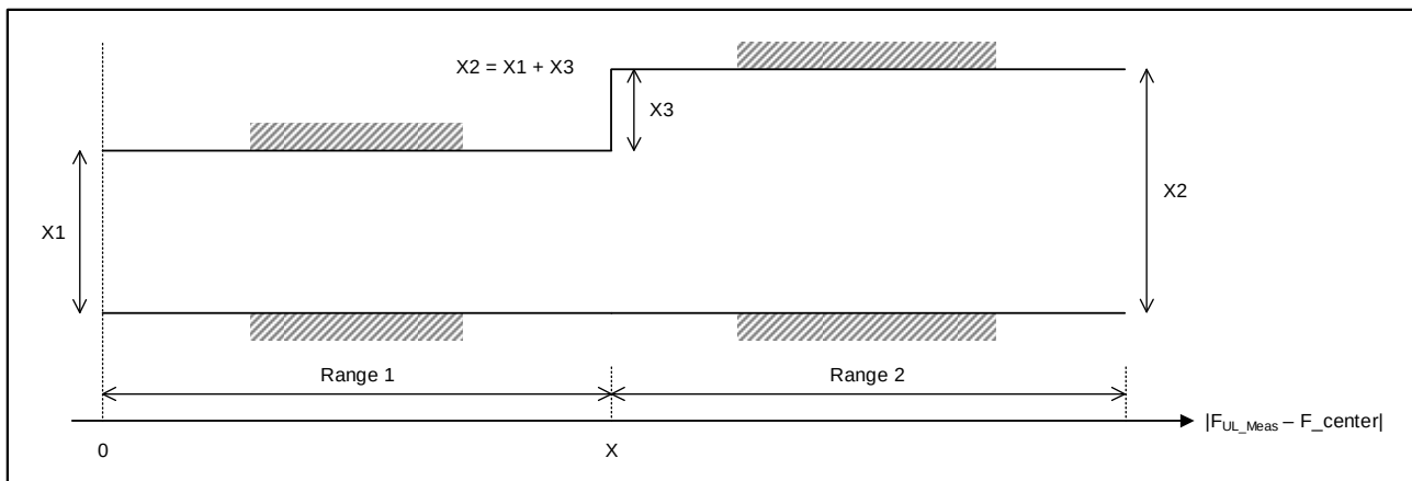
Figure 6.4D.2.5.5-1: The limits for EVM equalizer spectral flatness with the maximum allowed variation. F_{\text{center}} denotes the centre frequency of the allocated block of PRBs
