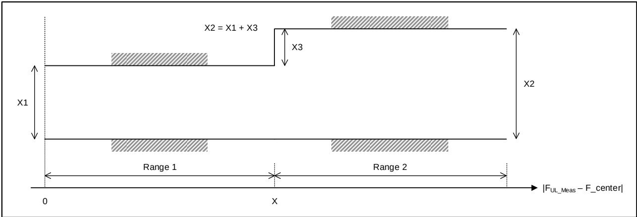
Figure 6.4.2.5.5-1: The limits for EVM equalizer spectral flatness with the maximum allowed variation. F_{center} denotes the centre frequency of the allocated block of PRBs
