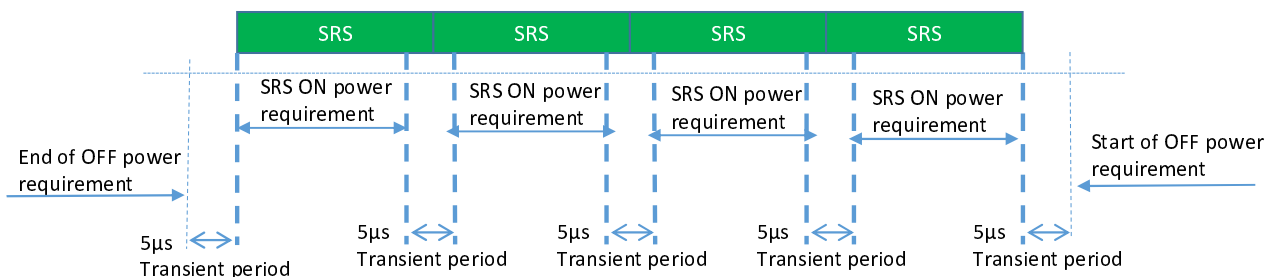
Figure 6.3.3.6.3-3: Consecutive SRS time mask for the case when power change is required and when 60kHz SCS is used in FR2
