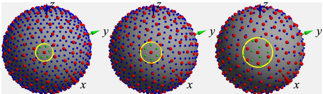
Figure M.2.2-5: Coarse & Fine Constant Density Grids for sample PC3 grids, left: 8x2, centre: 6x2, right: 4x2.
