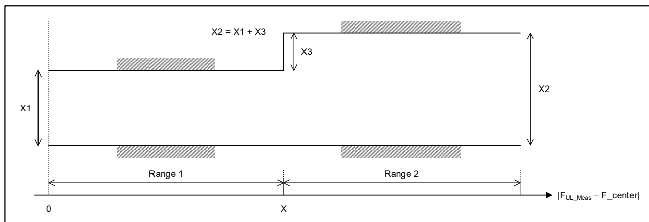
Figure 6.4.2.5.3-1: The limits for EVM equalizer spectral flatness with the maximum allowed variation. F_{\text{center}} denotes the centre frequency of the allocated block of PRBs. F_{\text{alloc}} denotes the bandwidth of the PRB allocation
