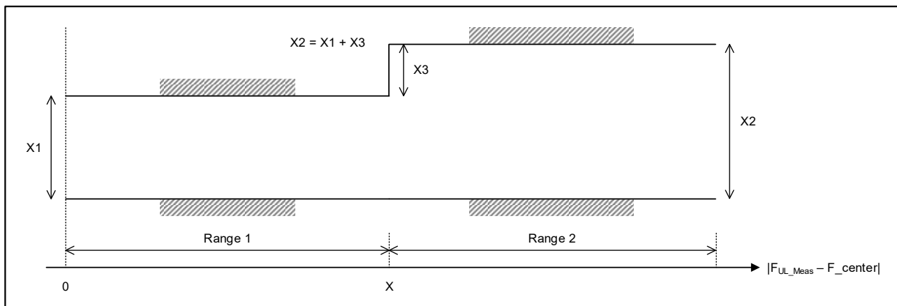
Figure 6.4D.2.5.5-1: The limits for EVM equalizer spectral flatness with the maximum allowed variation. F_{\text{center}} denotes the centre frequency of the allocated block of PRBs
