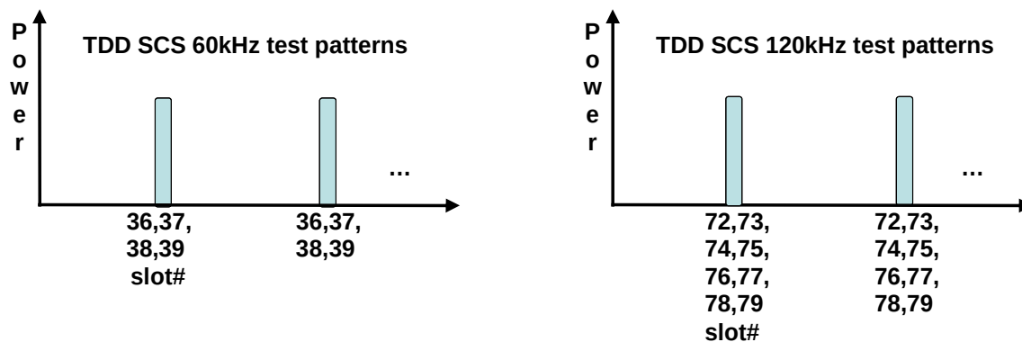
Figure 6.3.4.4.2-1: Test uplink transmission
