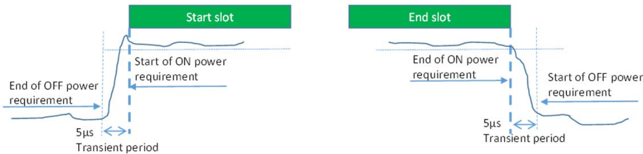
Figure 6.3.3.2.3-1: General ON/OFF time mask for NR UL transmission in FR2
