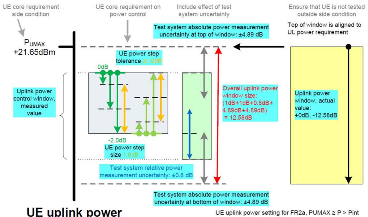
Figure F.4.3.2-1: Example NR FR2 uplink power setting to be below a requirement
