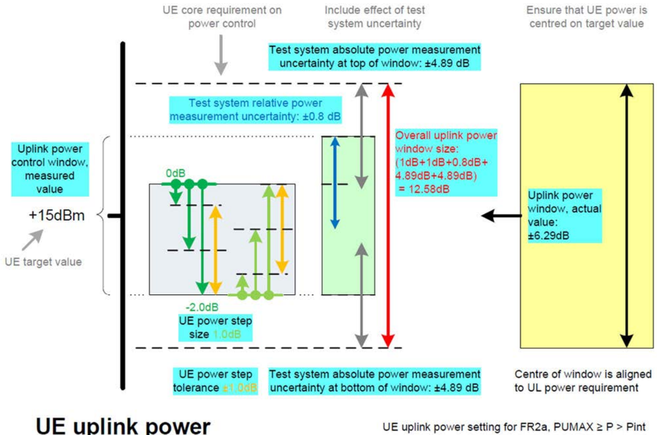
Figure F.4.4.2-1: Example NR FR2 uplink power setting centred on a target value
